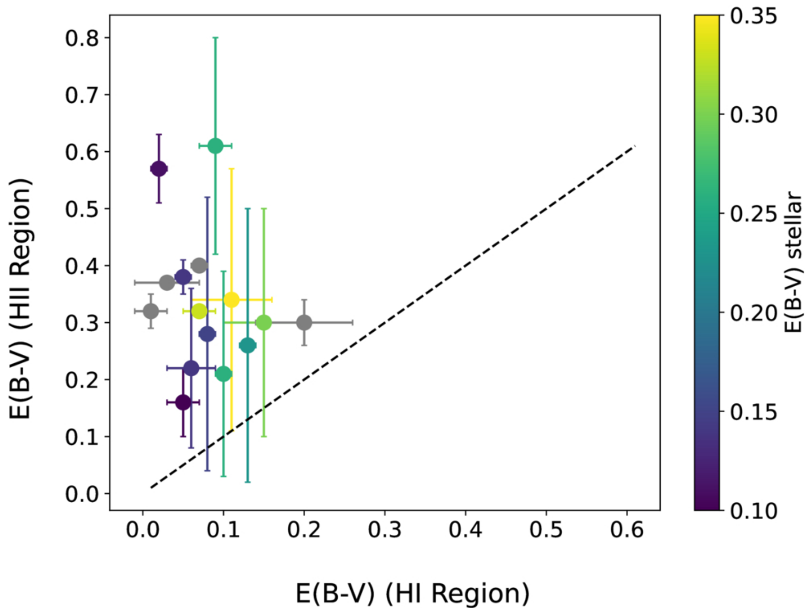
Figure 21. from Adarsh Ranjan et al 2026 Astron. J. 172 doi:10.3847/1538-3881/ae9943 https://dx.doi.org/10.3847/1538-3881/ae9943 © 2026. The Author(s). Published by the American Astronomical Society.
