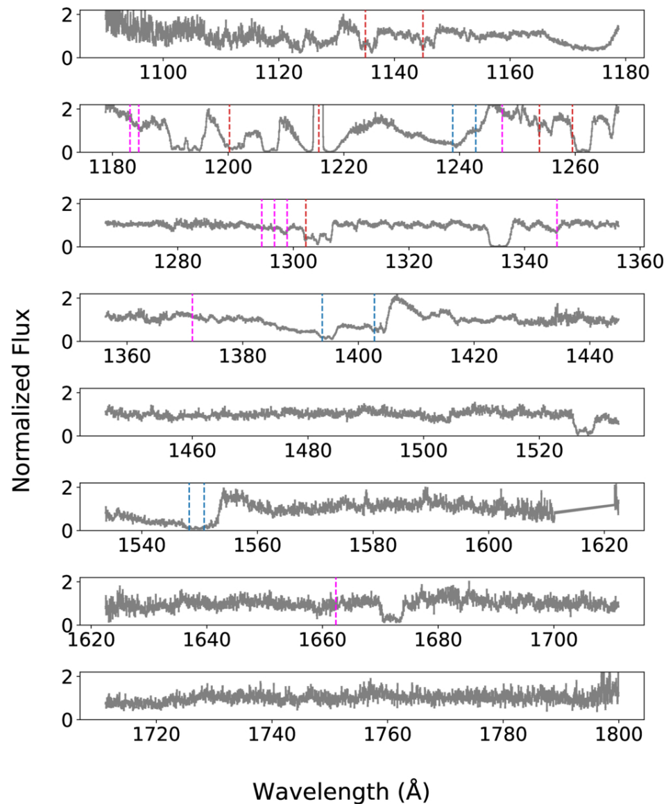
(a) HST/COS Spectra
