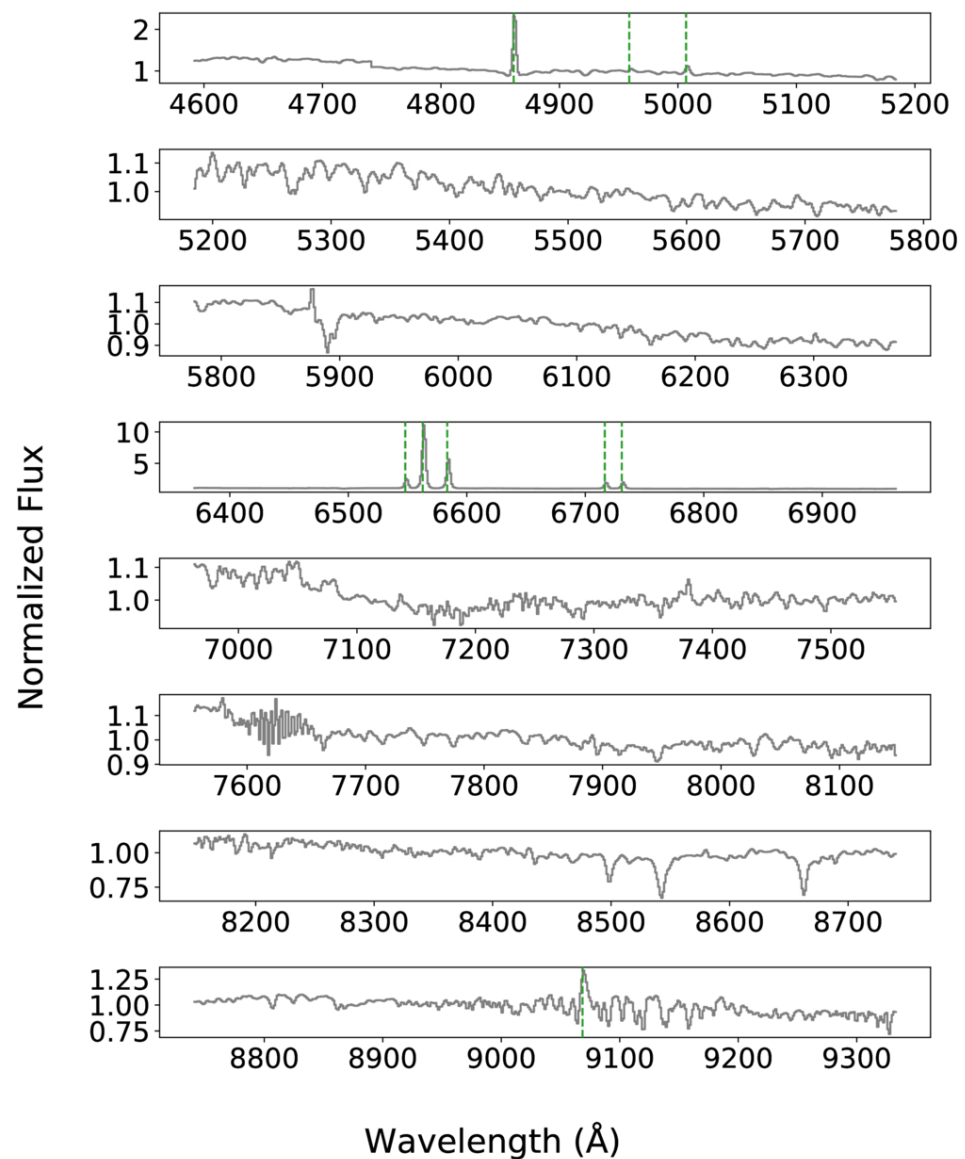
(b) VLT/MUSE Spectra
