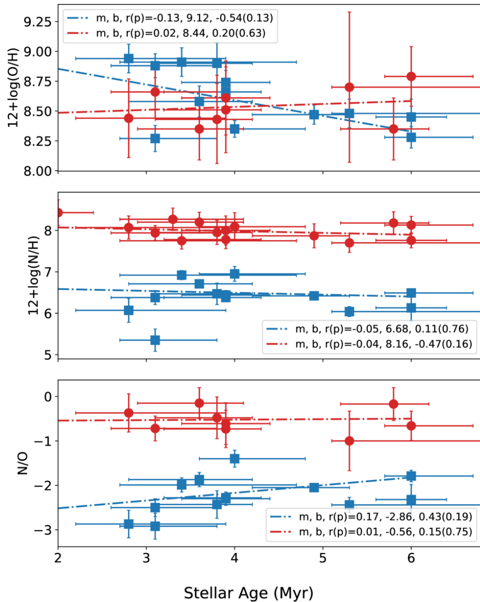
Figure 18. from Adarsh Ranjan et al 2026 Astron. J. 172 doi:10.3847/1538-3881/ae9943 https://dx.doi.org/10.3847/1538-3881/ae9943 © 2026. The Author(s). Published by the American Astronomical Society.
