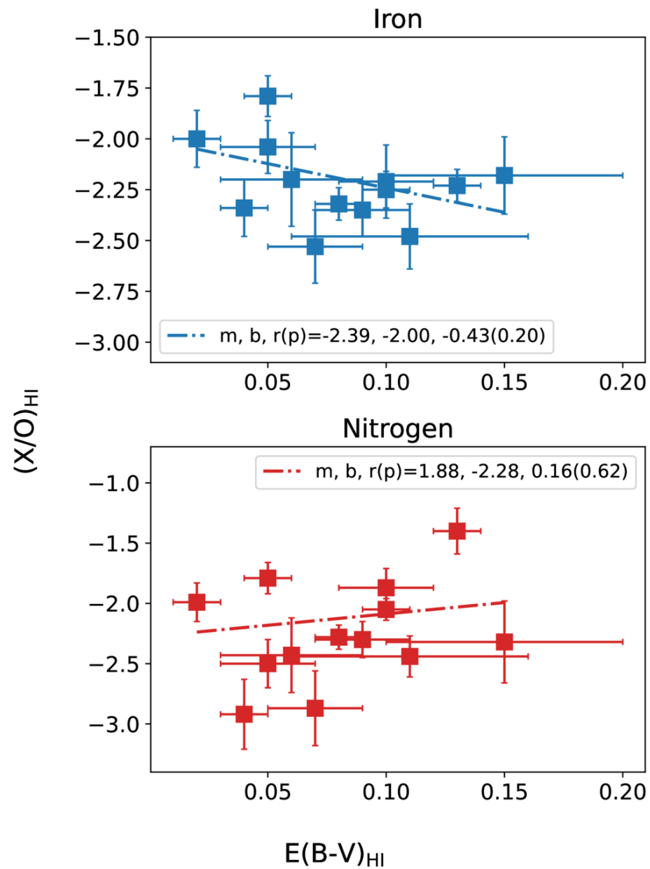
Figure 13. from Adarsh Ranjan et al 2026 Astron. J. 172 doi:10.3847/1538-3881/ae9943 https://dx.doi.org/10.3847/1538-3881/ae9943 © 2026. The Author(s). Published by the American Astronomical Society.
