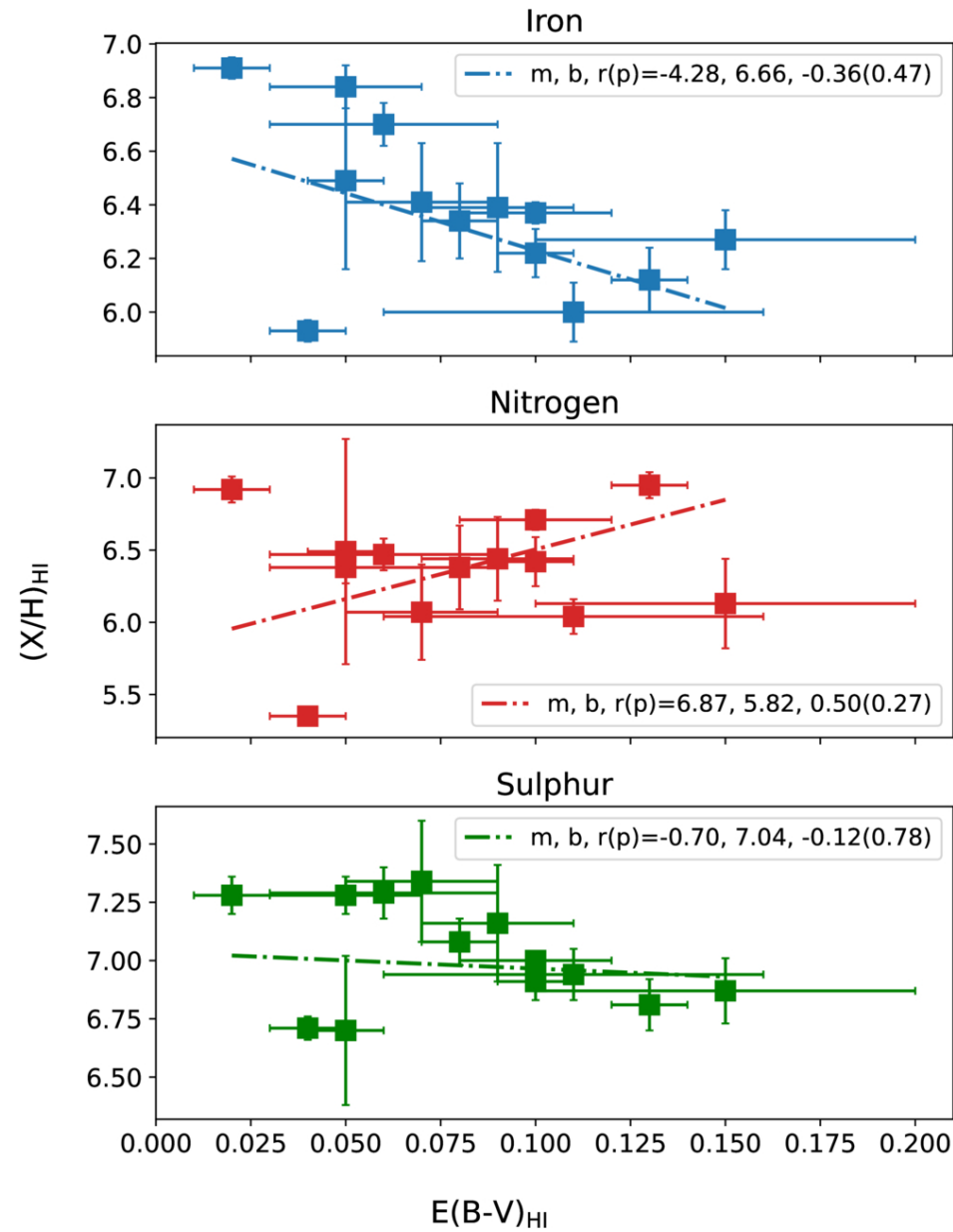
Figure 12. from Adarsh Ranjan et al 2026 Astron. J. 172 doi:10.3847/1538-3881/ae9943 https://dx.doi.org/10.3847/1538-3881/ae9943 © 2026. The Author(s). Published by the American Astronomical Society.
