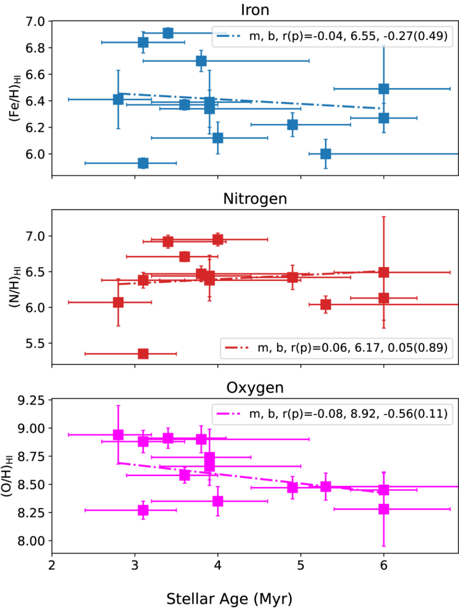
Figure 11. from Adarsh Ranjan et al 2026 Astron. J. 172 doi:10.3847/1538-3881/ae9943 https://dx.doi.org/10.3847/1538-3881/ae9943 © 2026. The Author(s). Published by the American Astronomical Society.
