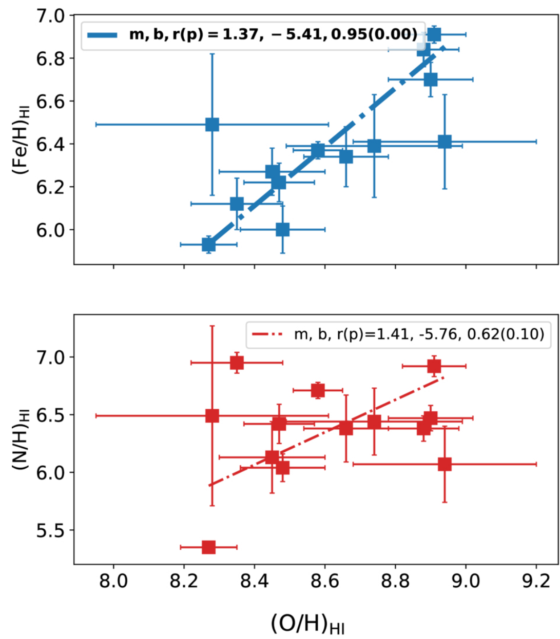
Figure 10. from Adarsh Ranjan et al 2026 Astron. J. 172 doi:10.3847/1538-3881/ae9943 https://dx.doi.org/10.3847/1538-3881/ae9943 © 2026. The Author(s). Published by the American Astronomical Society.
