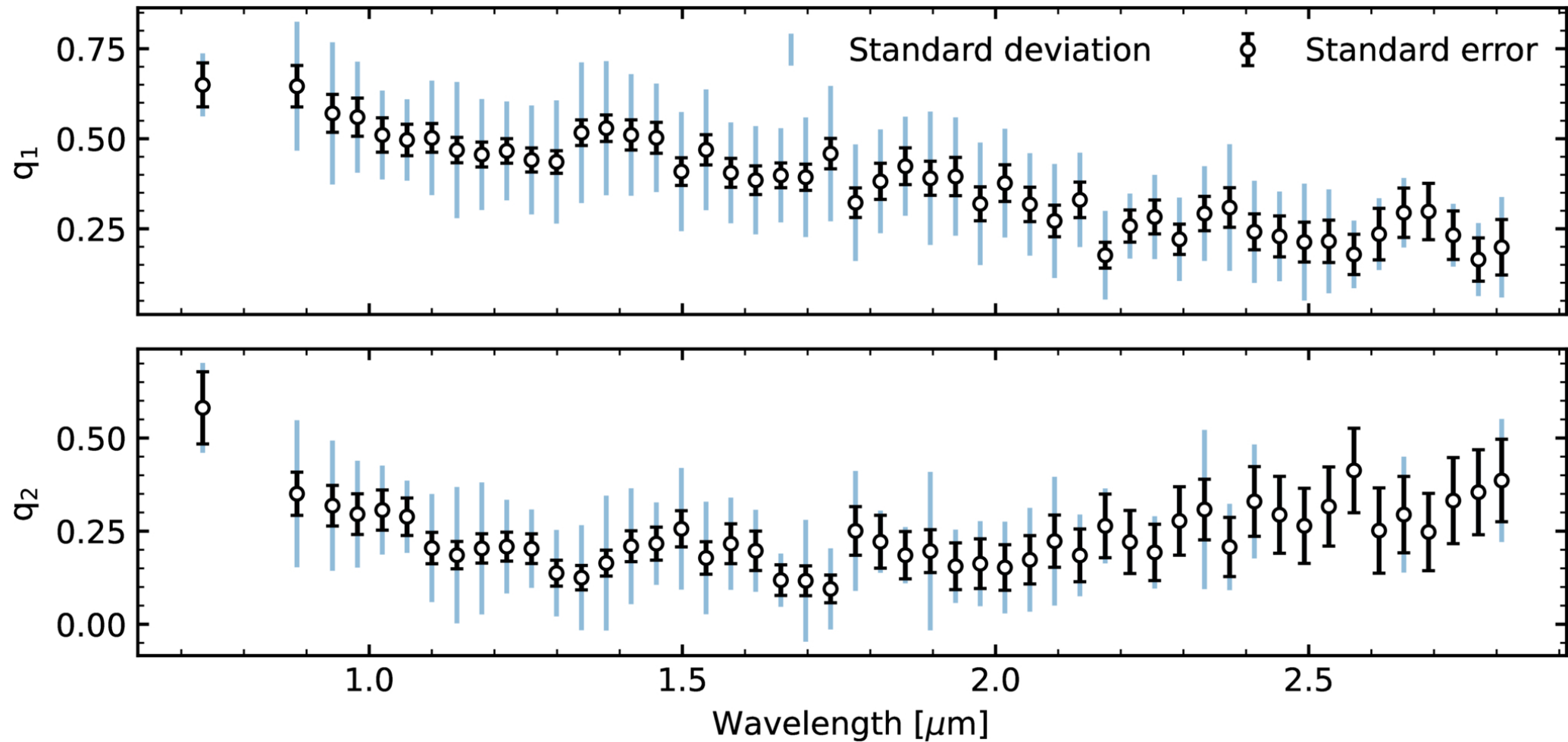
Figure B1. from Olivia Lim et al 2026 Astron. J. 172 doi:10.3847/1538-3881/ae990a https://dx.doi.org/10.3847/1538-3881/ae990a © 2026. The Author(s). Published by the American Astronomical Society.
