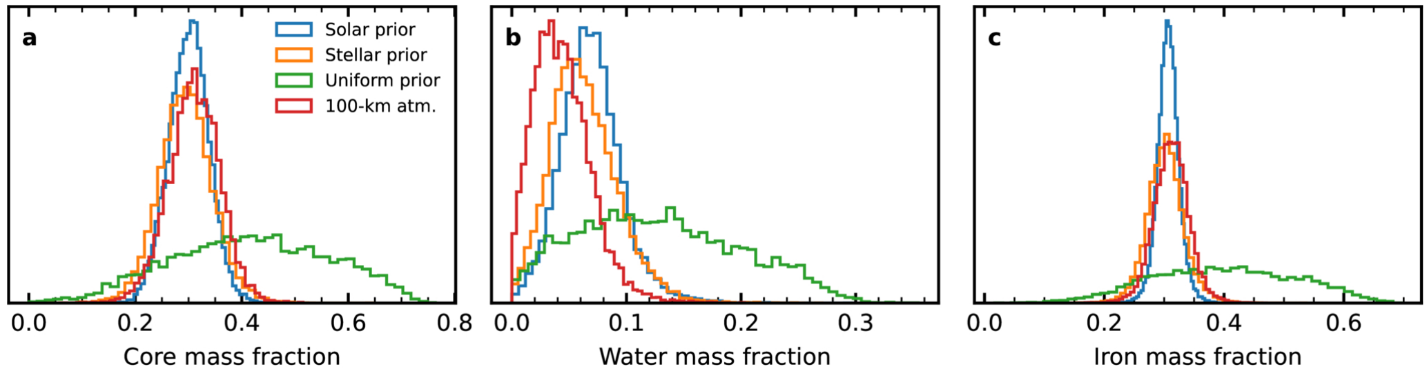
Figure 4. from Olivia Lim et al 2026 Astron. J. 172 doi:10.3847/1538-3881/ae990a https://dx.doi.org/10.3847/1538-3881/ae990a © 2026. The Author(s). Published by the American Astronomical Society.
