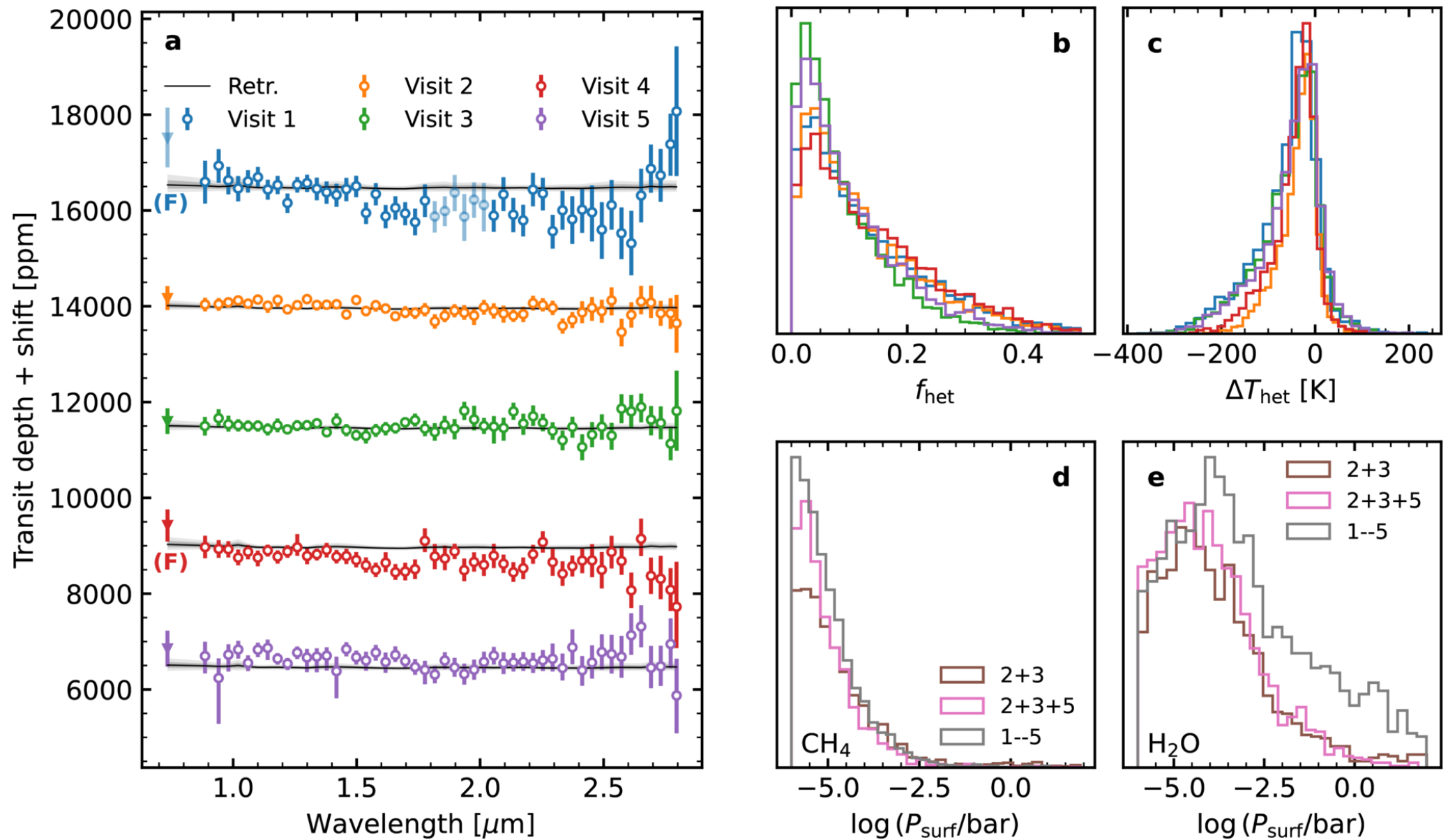
Figure 2. from Olivia Lim et al 2026 Astron. J. 172 doi:10.3847/1538-3881/ae990a https://dx.doi.org/10.3847/1538-3881/ae990a © 2026. The Author(s). Published by the American Astronomical Society.
