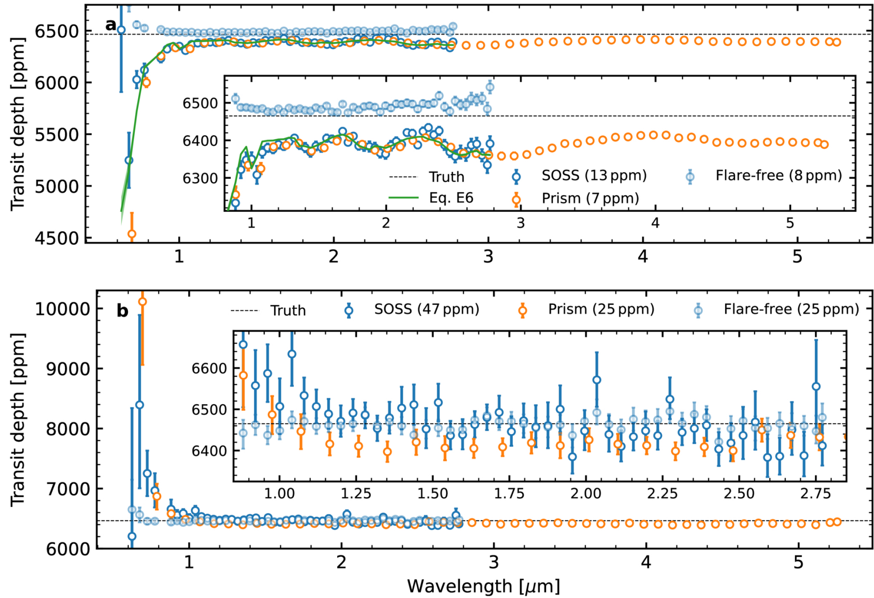
Figure E2. from Olivia Lim et al 2026 Astron. J. 172 doi:10.3847/1538-3881/ae990a https://dx.doi.org/10.3847/1538-3881/ae990a © 2026. The Author(s). Published by the American Astronomical Society.
