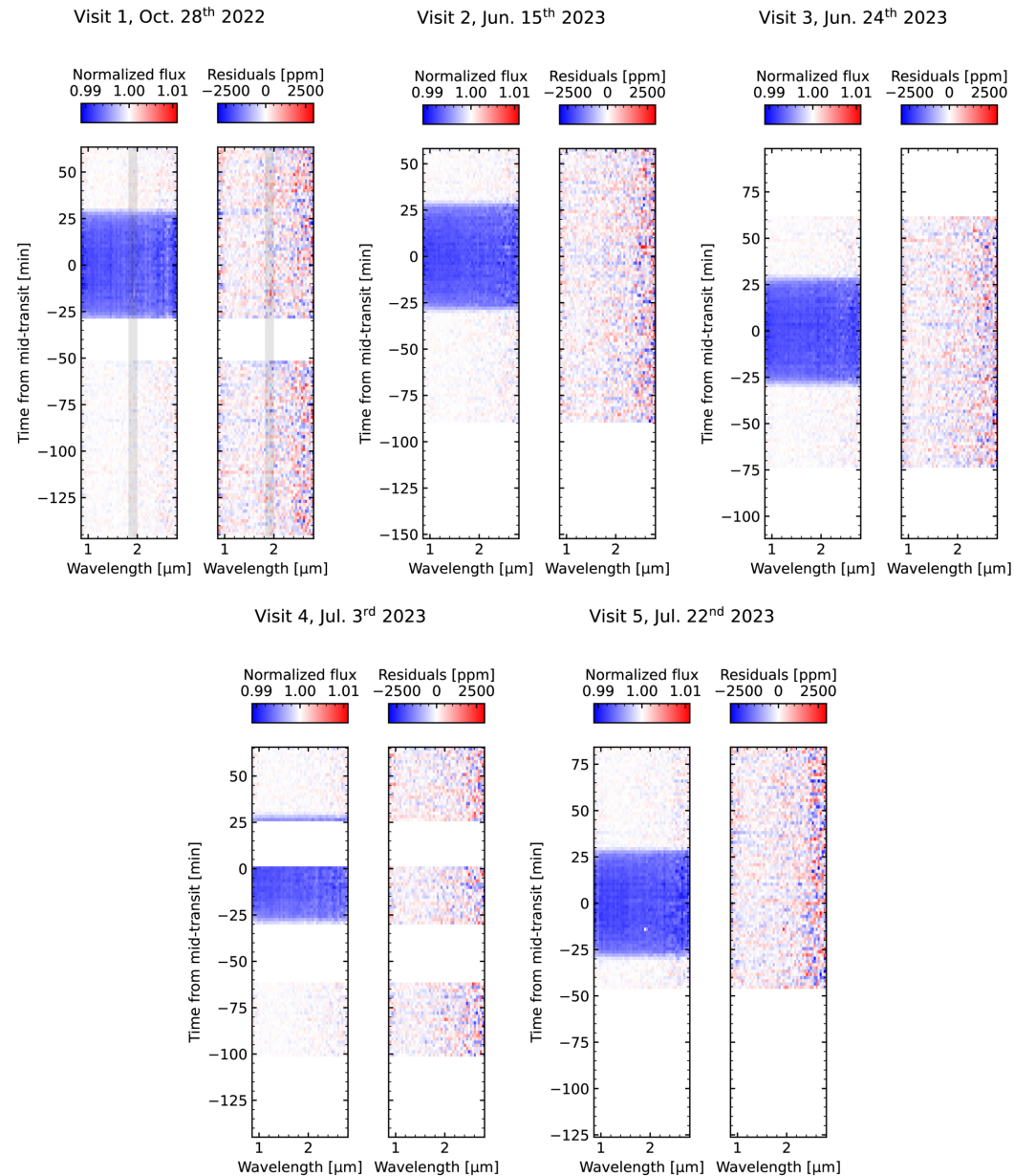
Figure B6. from Olivia Lim et al 2026 Astron. J. 172 doi:10.3847/1538-3881/ae990a https://dx.doi.org/10.3847/1538-3881/ae990a © 2026. The Author(s). Published by the American Astronomical Society.
