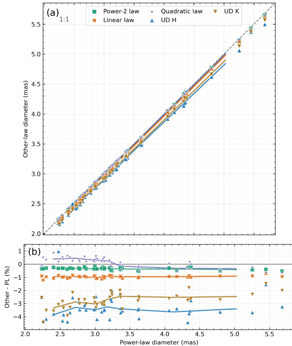
Figure 9. from Narsireddy Anugu et al 2026 Astron. J. 172 doi:10.3847/1538-3881/ae9878 https://dx.doi.org/10.3847/1538-3881/ae9878 © 2026. The Author(s). Published by the American Astronomical Society.
