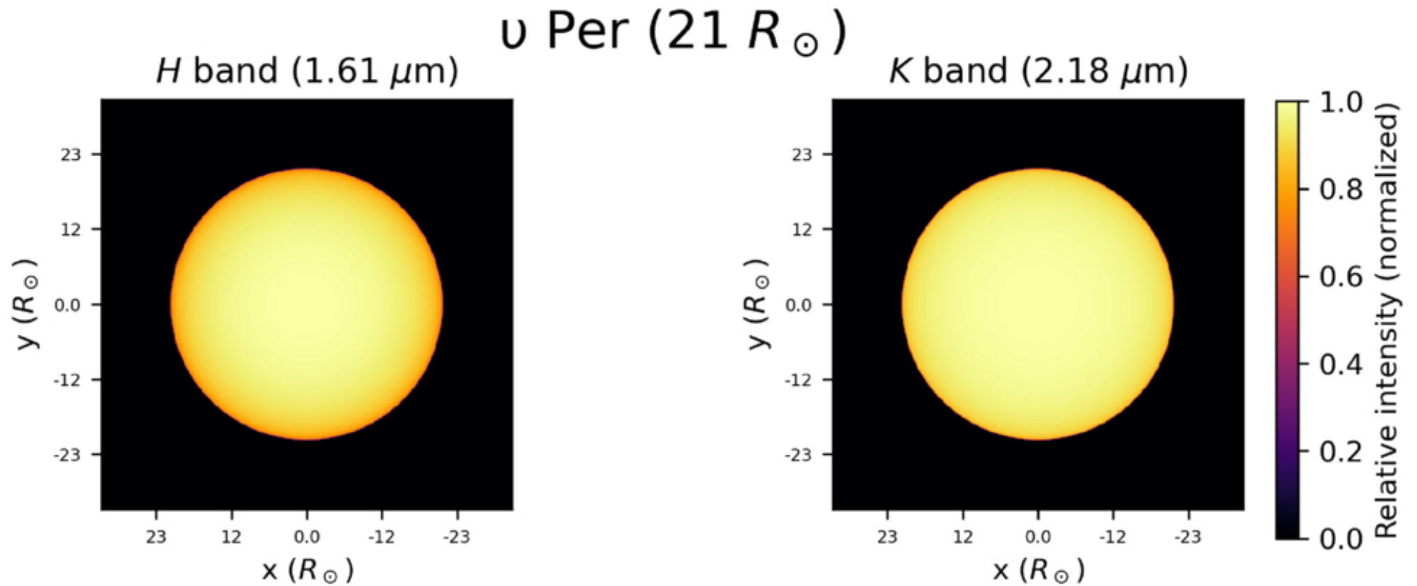
Figure 8. Power-law limb-darkening model images on a physical-radius scale from Narsireddy Anugu et al 2026 Astron. J. 172 doi:10.3847/1538-3881/ae9878 https://dx.doi.org/10.3847/1538-3881/ae9878 © 2026. The Author(s). Published by the American Astronomical Society.
