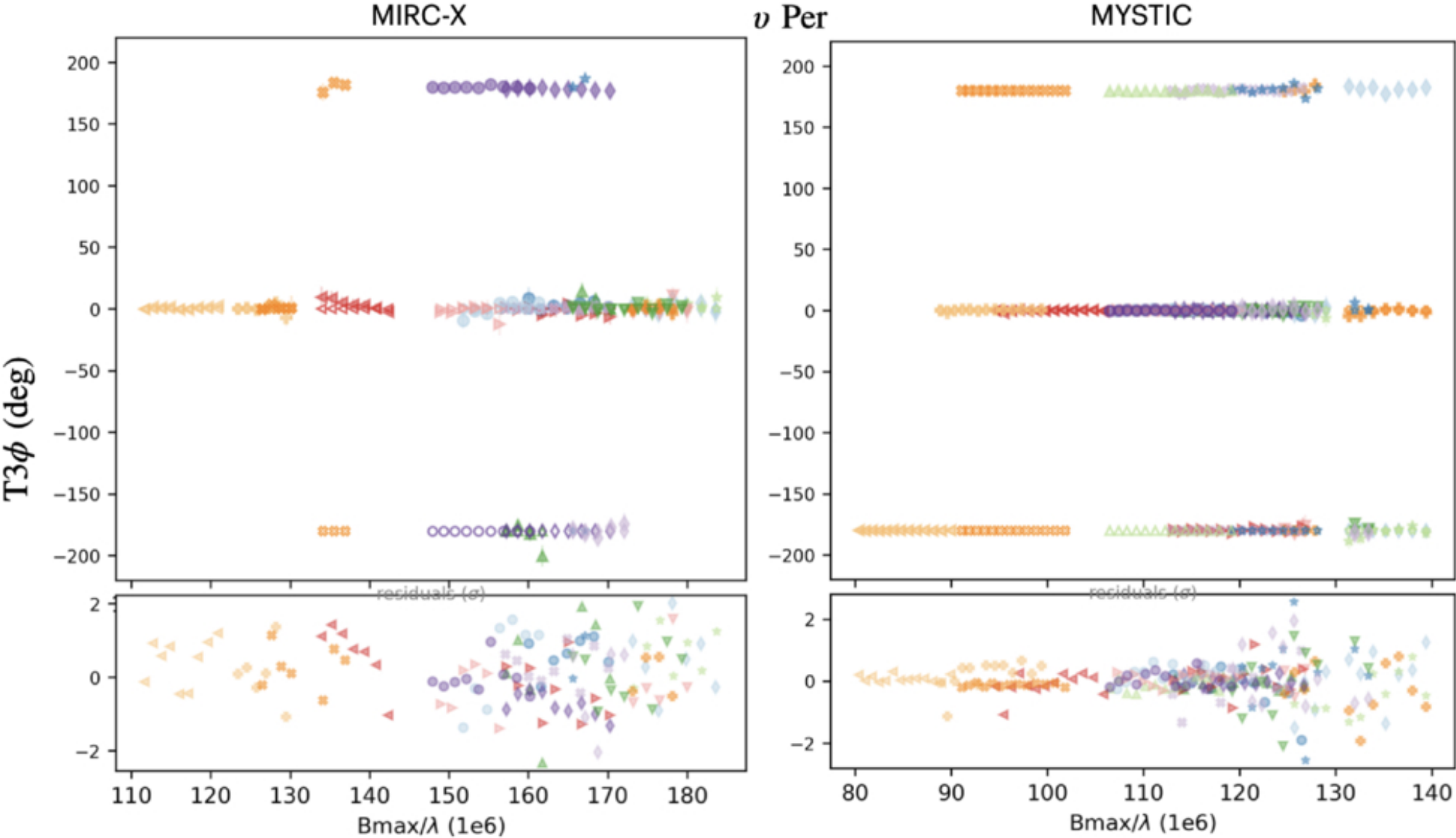
Figure 7. Closure-phase and companion-search diagnostics from Narsireddy Anugu et al 2026 Astron. J. 172 doi:10.3847/1538-3881/ae9878 https://dx.doi.org/10.3847/1538-3881/ae9878 © 2026. The Author(s). Published by the American Astronomical Society.
