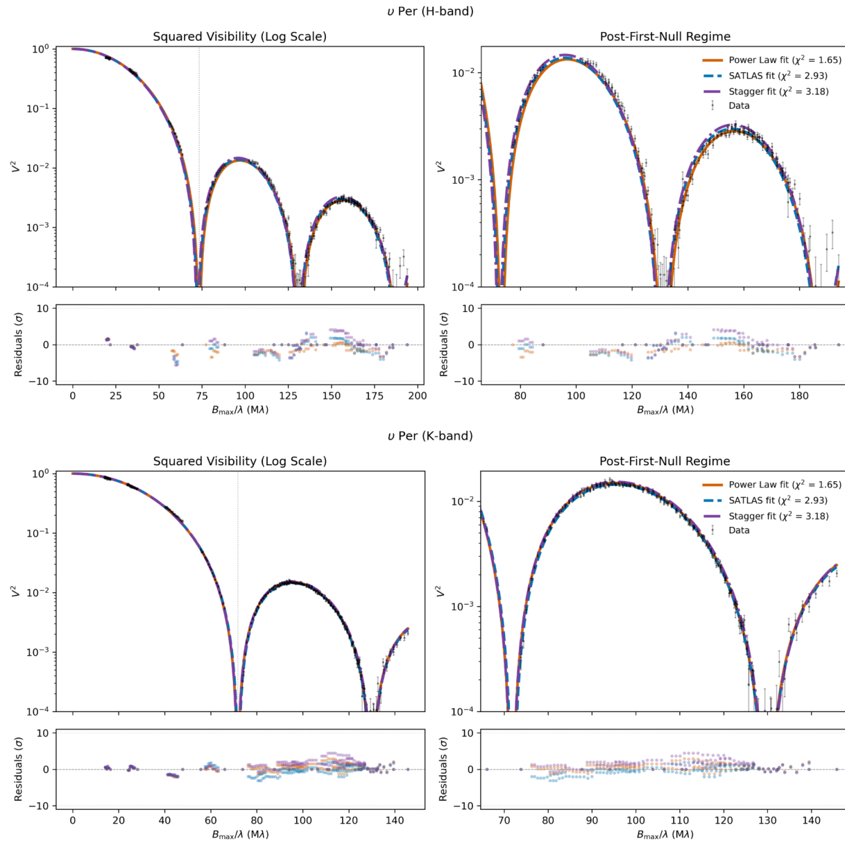
Figure 6. Data-vs.-model comparisons for the limb-darkening fits from Narsireddy Anugu et al 2026 Astron. J. 172 doi:10.3847/1538-3881/ae9878 https://dx.doi.org/10.3847/1538-3881/ae9878 © 2026. The Author(s). Published by the American Astronomical Society.
