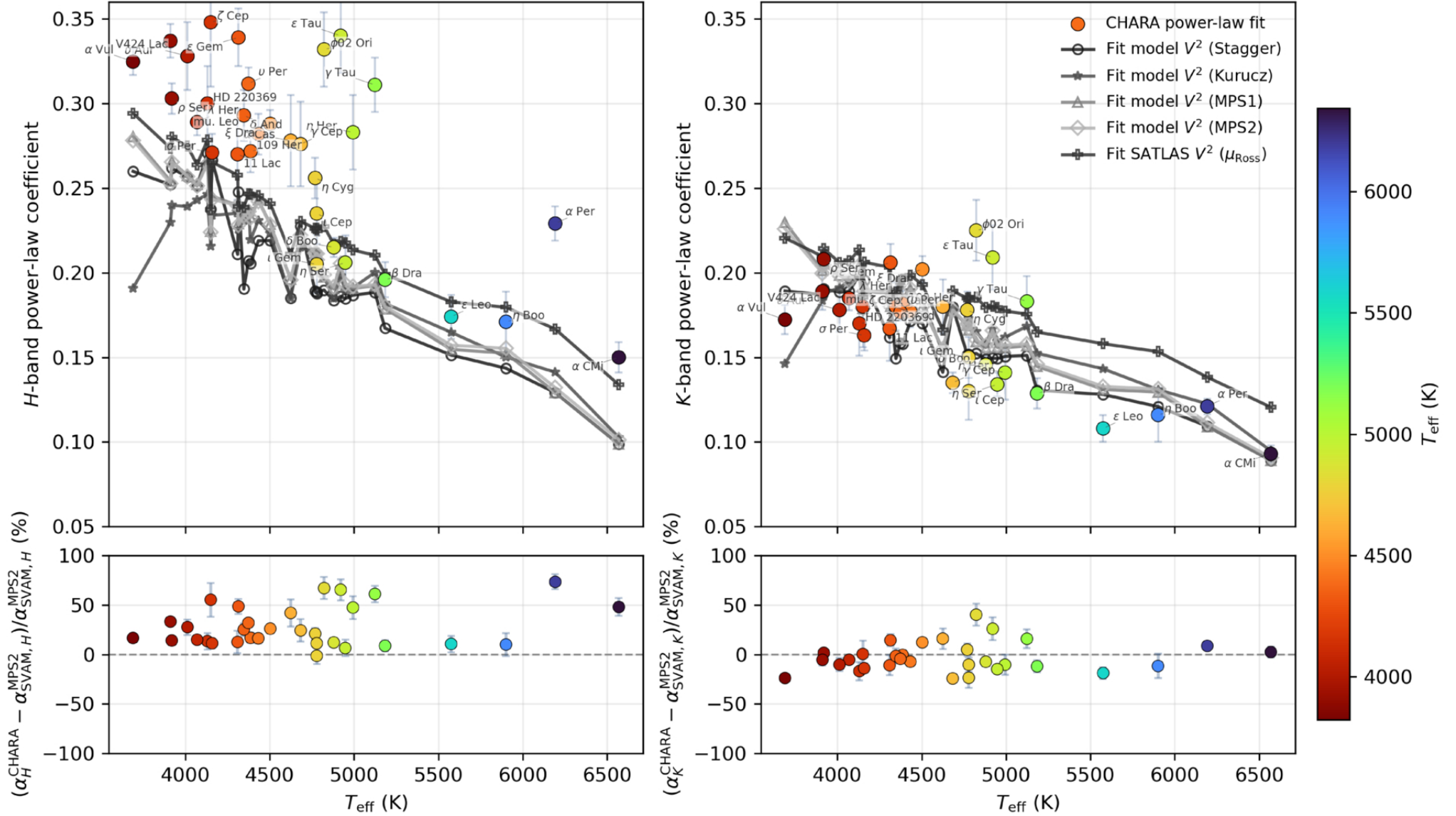
Figure 5. from Narsireddy Anugu et al 2026 Astron. J. 172 doi:10.3847/1538-3881/ae9878 https://dx.doi.org/10.3847/1538-3881/ae9878 © 2026. The Author(s). Published by the American Astronomical Society.
