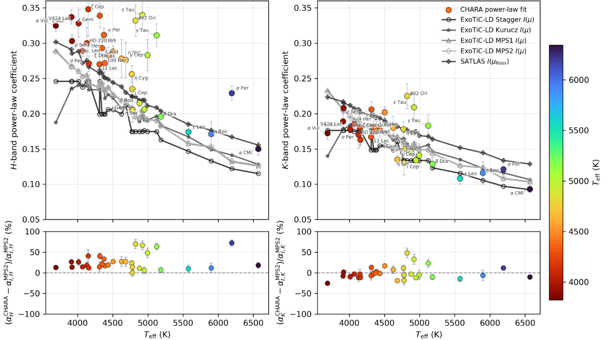
Figure 4. from Narsireddy Anugu et al 2026 Astron. J. 172 doi:10.3847/1538-3881/ae9878 https://dx.doi.org/10.3847/1538-3881/ae9878 © 2026. The Author(s). Published by the American Astronomical Society.
