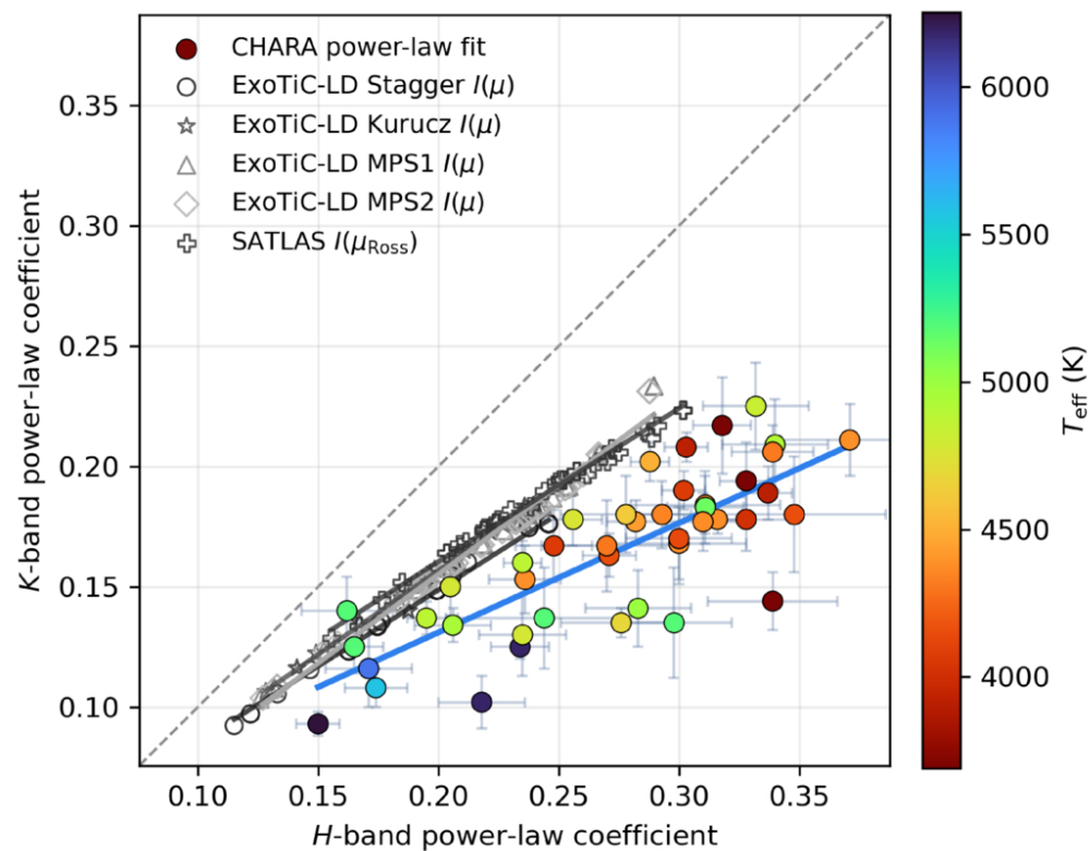
Figure 3. from Narsireddy Anugu et al 2026 Astron. J. 172 doi:10.3847/1538-3881/ae9878 https://dx.doi.org/10.3847/1538-3881/ae9878 © 2026. The Author(s). Published by the American Astronomical Society.
