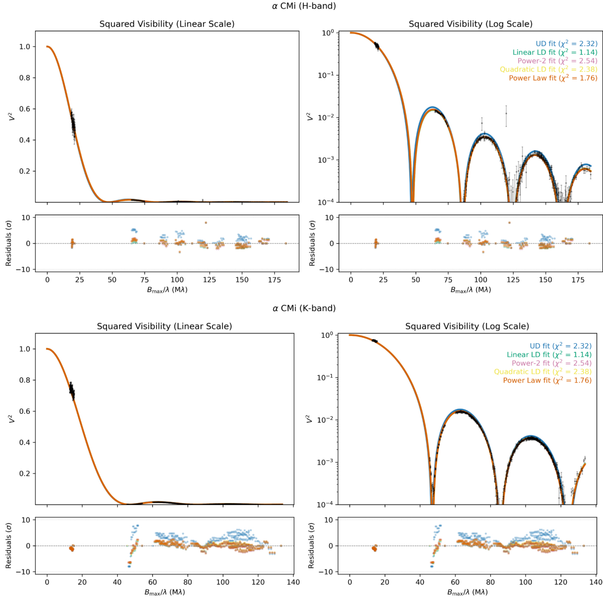
Figure 2. CHARA squared-visibility fits for the limb-darkening laws from Narsireddy Anugu et al 2026 Astron. J. 172 doi:10.3847/1538-3881/ae9878 https://dx.doi.org/10.3847/1538-3881/ae9878 © 2026. The Author(s). Published by the American Astronomical Society.
