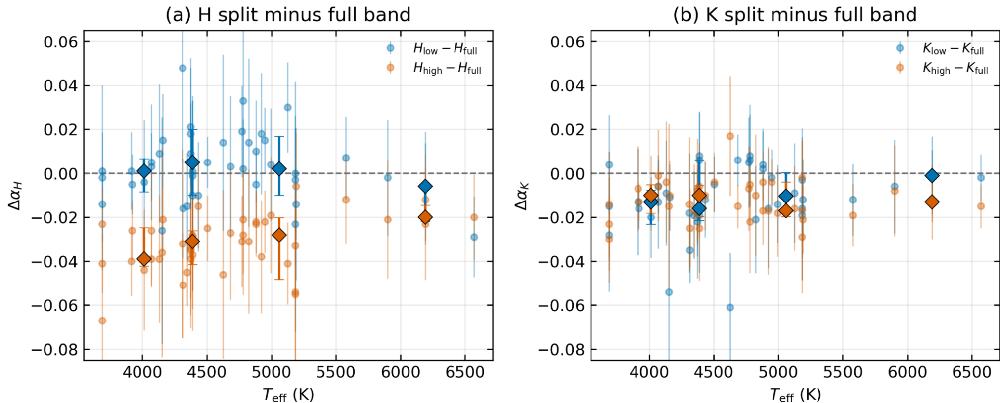
Figure D1. from Narsireddy Anugu et al 2026 Astron. J. 172 doi:10.3847/1538-3881/ae9878 https://dx.doi.org/10.3847/1538-3881/ae9878 © 2026. The Author(s). Published by the American Astronomical Society.
