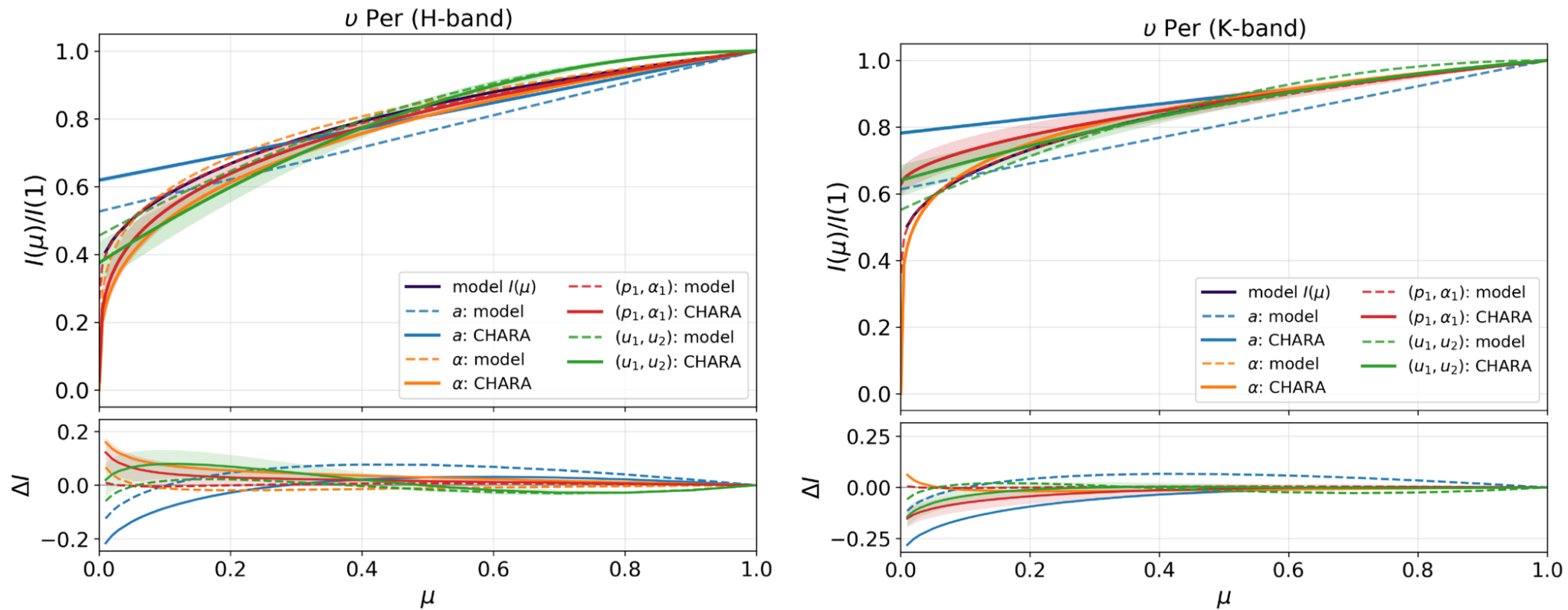
Figure C1. CHARA and model intensity-space comparisons from Narsireddy Anugu et al 2026 Astron. J. 172 doi:10.3847/1538-3881/ae9878 https://dx.doi.org/10.3847/1538-3881/ae9878 © 2026. The Author(s). Published by the American Astronomical Society.
