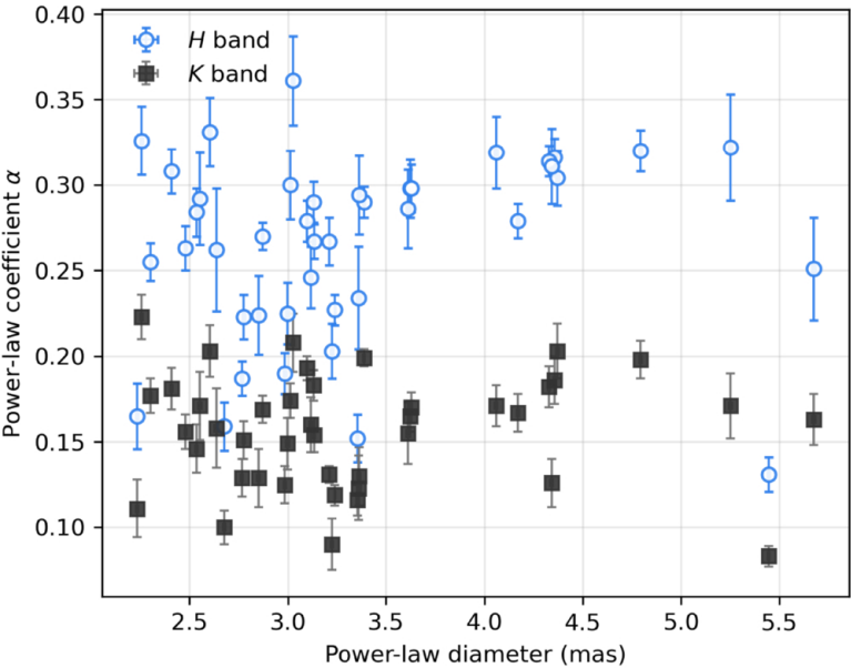
Figure B1. from Narsireddy Anugu et al 2026 Astron. J. 172 doi:10.3847/1538-3881/ae9878 https://dx.doi.org/10.3847/1538-3881/ae9878 © 2026. The Author(s). Published by the American Astronomical Society.
