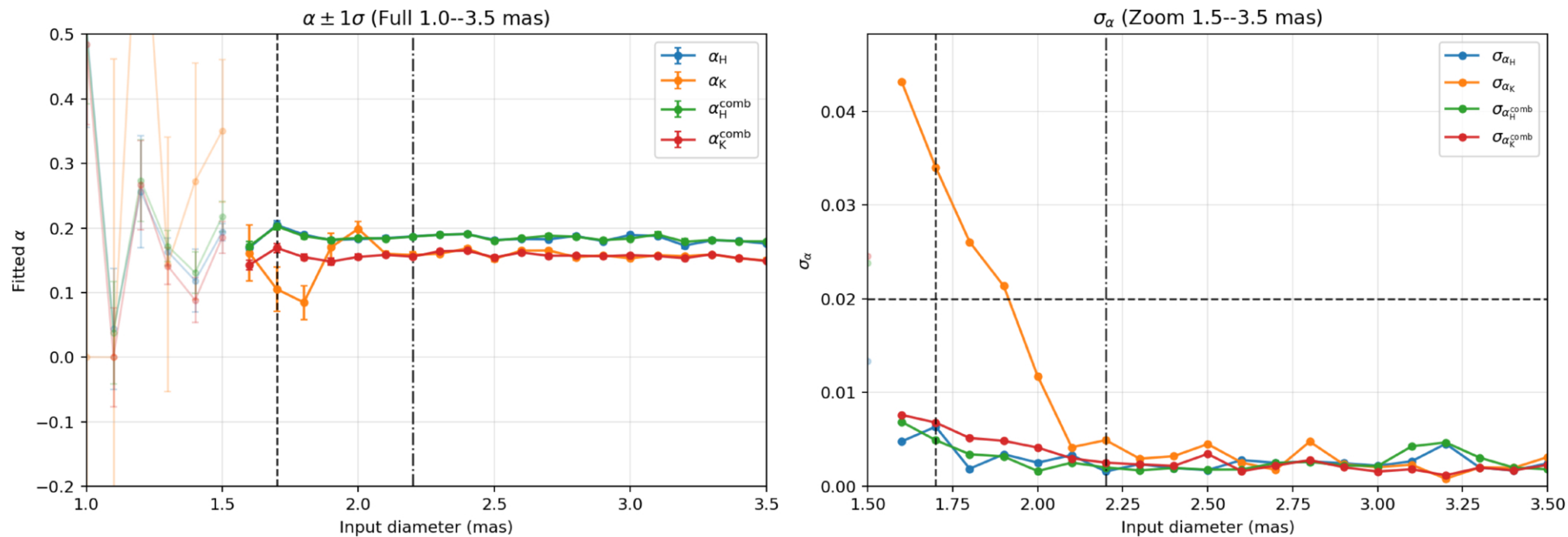
Figure A1. from Narsireddy Anugu et al 2026 Astron. J. 172 doi:10.3847/1538-3881/ae9878 https://dx.doi.org/10.3847/1538-3881/ae9878 © 2026. The Author(s). Published by the American Astronomical Society.
