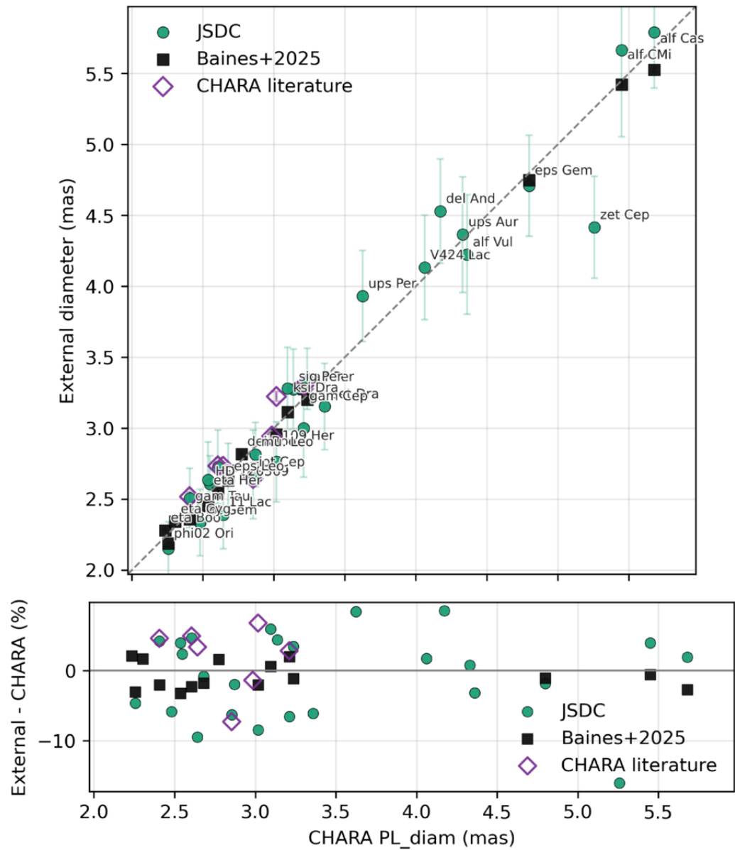
Figure 12. from Narsireddy Anugu et al 2026 Astron. J. 172 doi:10.3847/1538-3881/ae9878 https://dx.doi.org/10.3847/1538-3881/ae9878 © 2026. The Author(s). Published by the American Astronomical Society.
