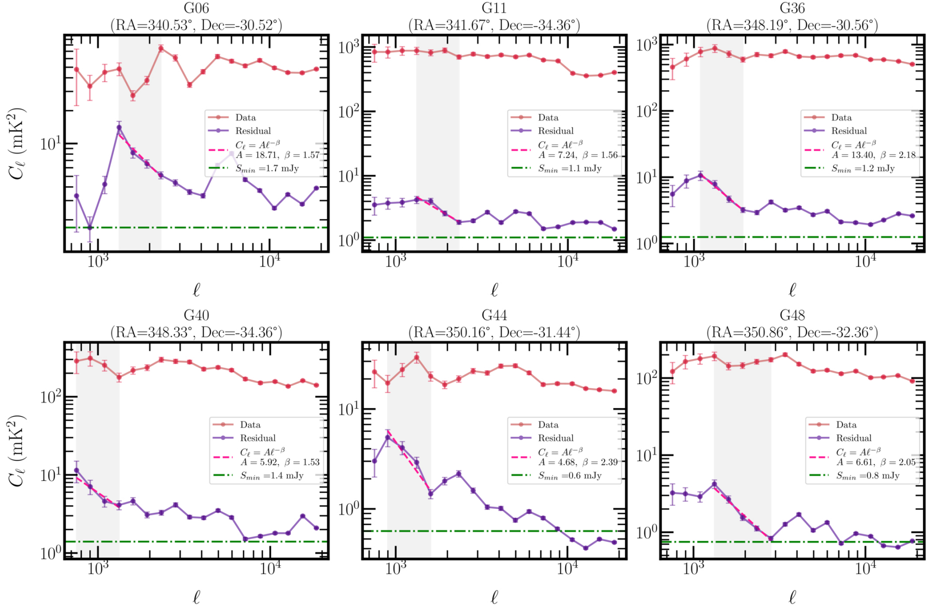
Figure 9. from Rashmi Sagar et al 2026 Astron. J. 172 doi:10.3847/1538-3881/ae9872 https://dx.doi.org/10.3847/1538-3881/ae9872 © 2026. The Author(s). Published by the American Astronomical Society.
