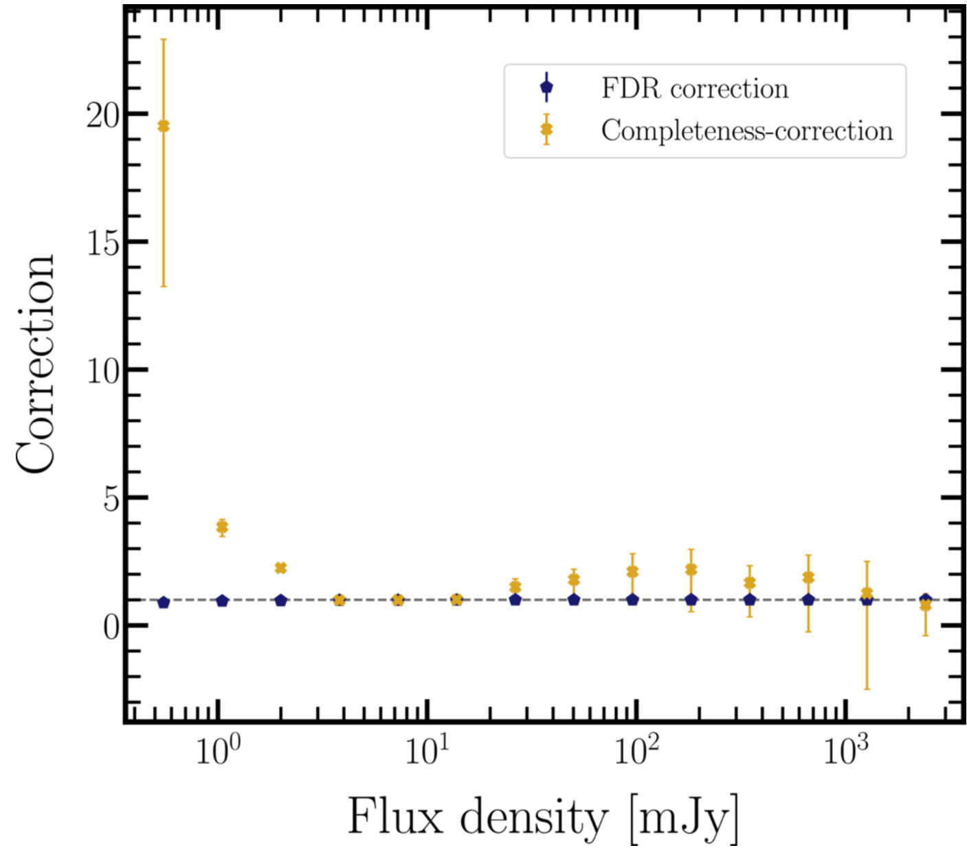
Figure 7. from Rashmi Sagar et al 2026 Astron. J. 172 doi:10.3847/1538-3881/ae9872 https://dx.doi.org/10.3847/1538-3881/ae9872 © 2026. The Author(s). Published by the American Astronomical Society.
