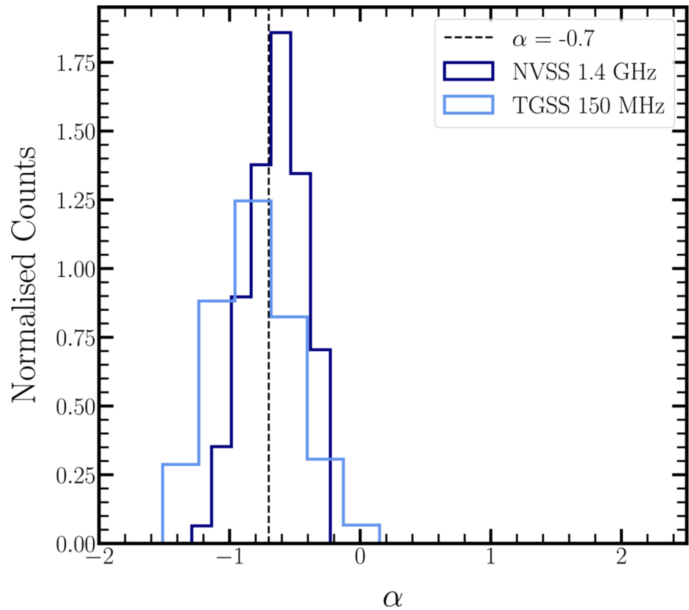
Figure 6. from Rashmi Sagar et al 2026 Astron. J. 172 doi:10.3847/1538-3881/ae9872 https://dx.doi.org/10.3847/1538-3881/ae9872 © 2026. The Author(s). Published by the American Astronomical Society.
