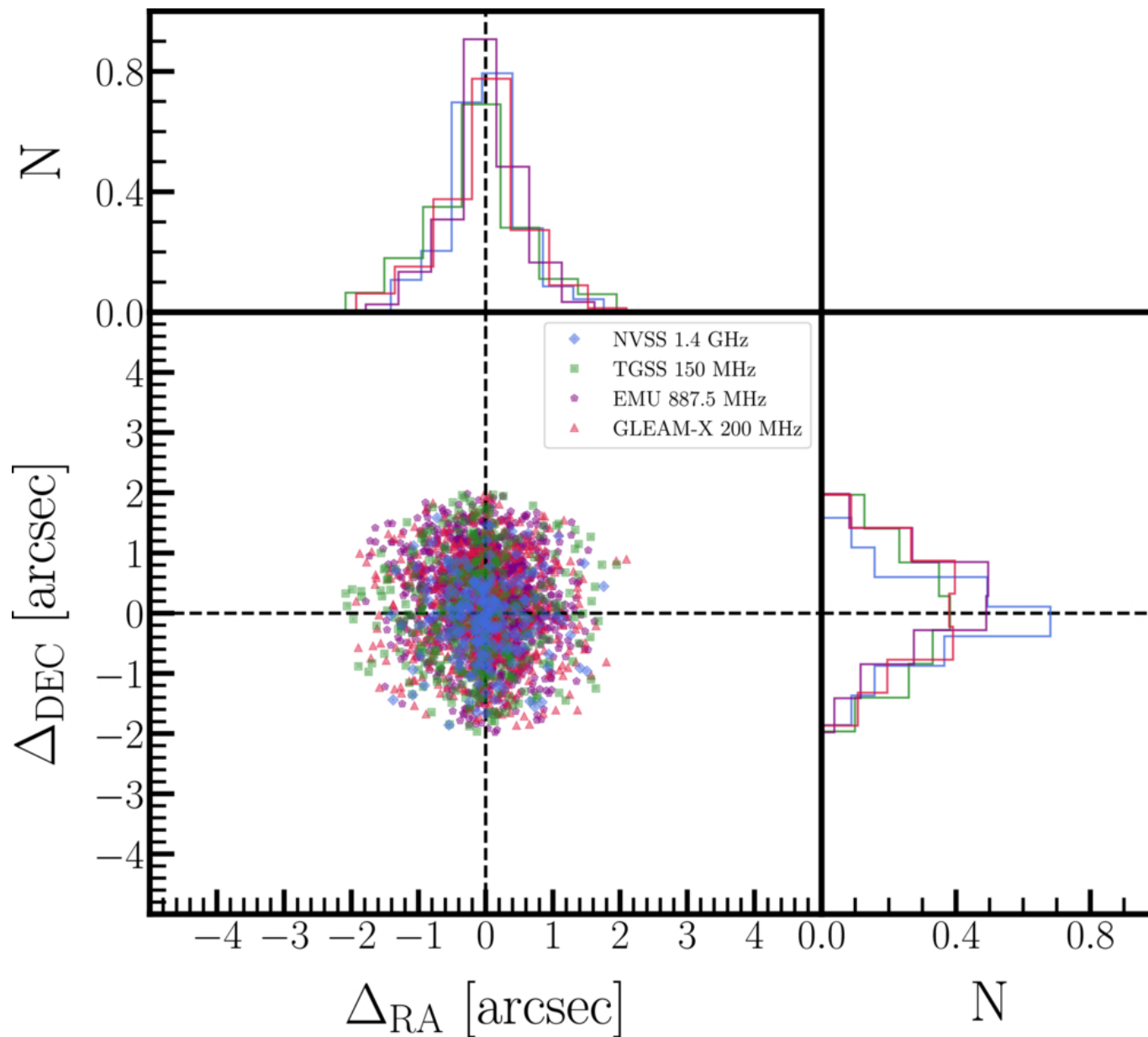
Figure 5. from Rashmi Sagar et al 2026 Astron. J. 172 doi:10.3847/1538-3881/ae9872 https://dx.doi.org/10.3847/1538-3881/ae9872 © 2026. The Author(s). Published by the American Astronomical Society.
