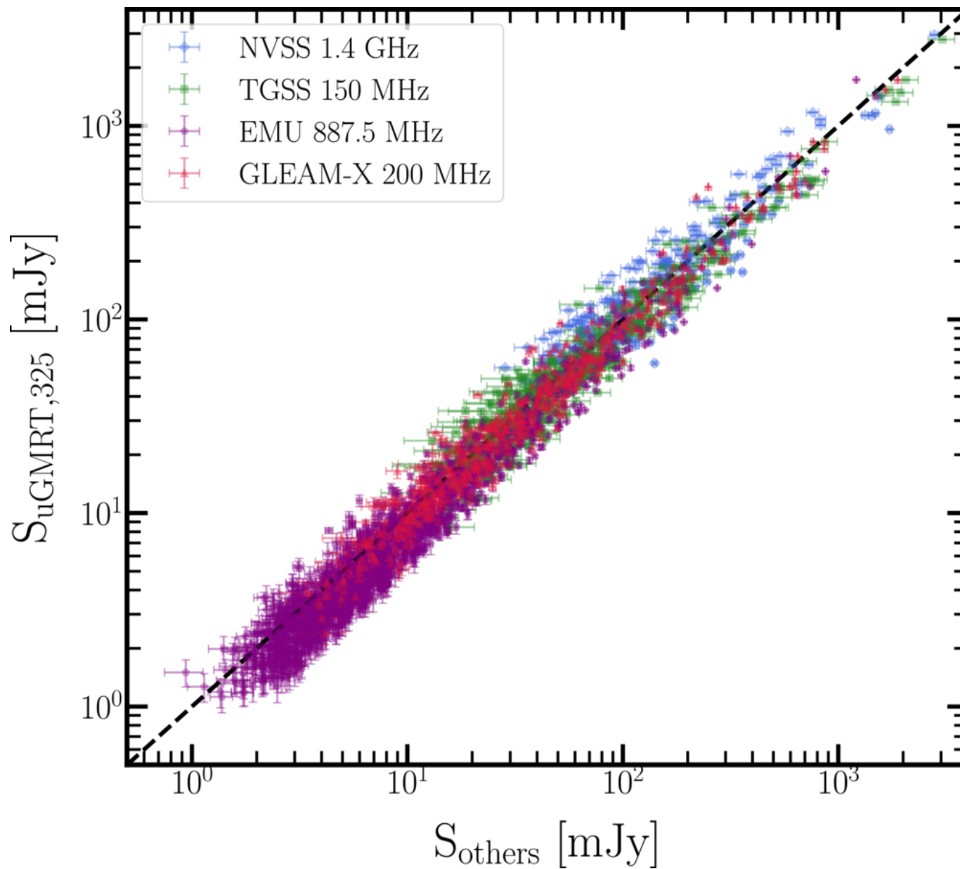
Figure 4. from Rashmi Sagar et al 2026 Astron. J. 172 doi:10.3847/1538-3881/ae9872 https://dx.doi.org/10.3847/1538-3881/ae9872 © 2026. The Author(s). Published by the American Astronomical Society.
