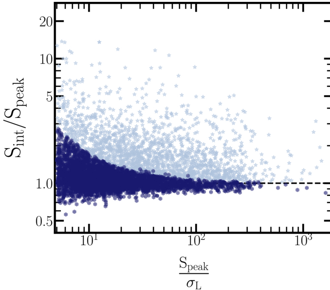
Figure 3. from Rashmi Sagar et al 2026 Astron. J. 172 doi:10.3847/1538-3881/ae9872 https://dx.doi.org/10.3847/1538-3881/ae9872 © 2026. The Author(s). Published by the American Astronomical Society.
