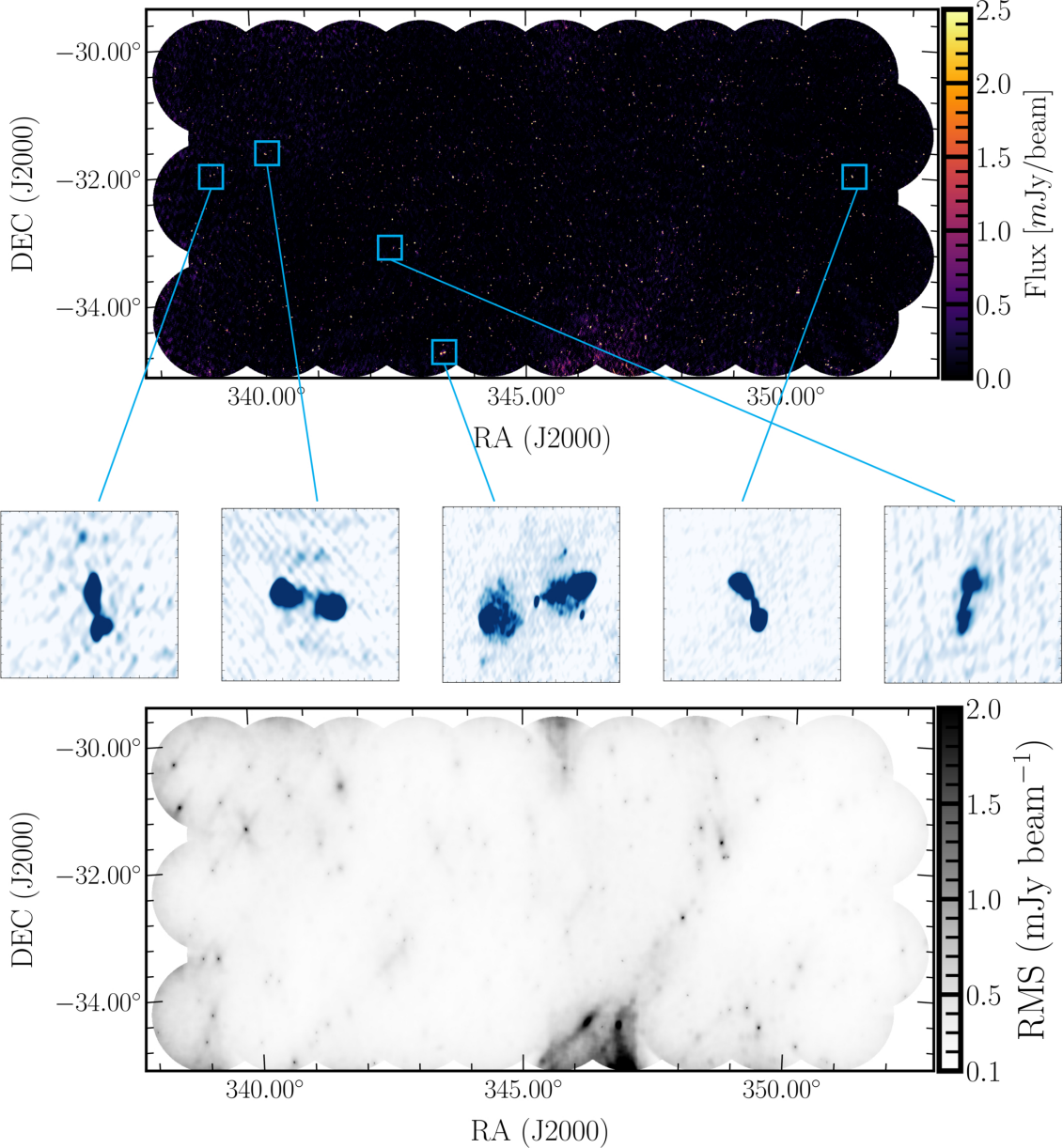
Figure 2. from Rashmi Sagar et al 2026 Astron. J. 172 doi:10.3847/1538-3881/ae9872 https://dx.doi.org/10.3847/1538-3881/ae9872 © 2026. The Author(s). Published by the American Astronomical Society.
