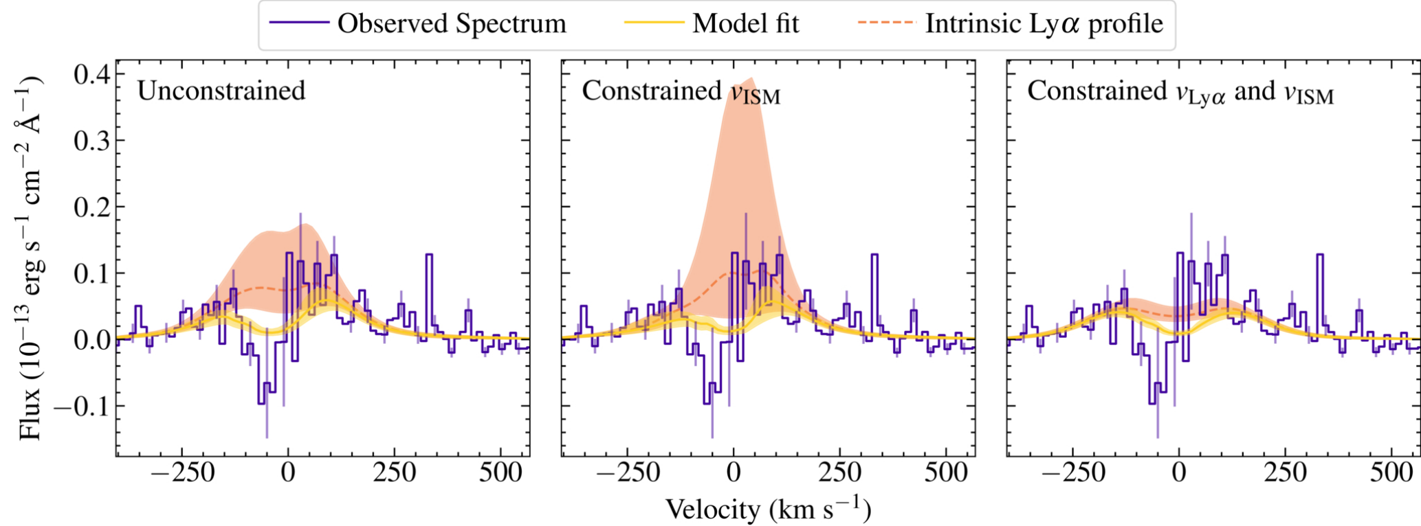
Figure 8. from Cyril Gapp et al 2026 Astron. J. 172 doi:10.3847/1538-3881/ae9866 https://dx.doi.org/10.3847/1538-3881/ae9866 © 2026. The Author(s). Published by the American Astronomical Society.
