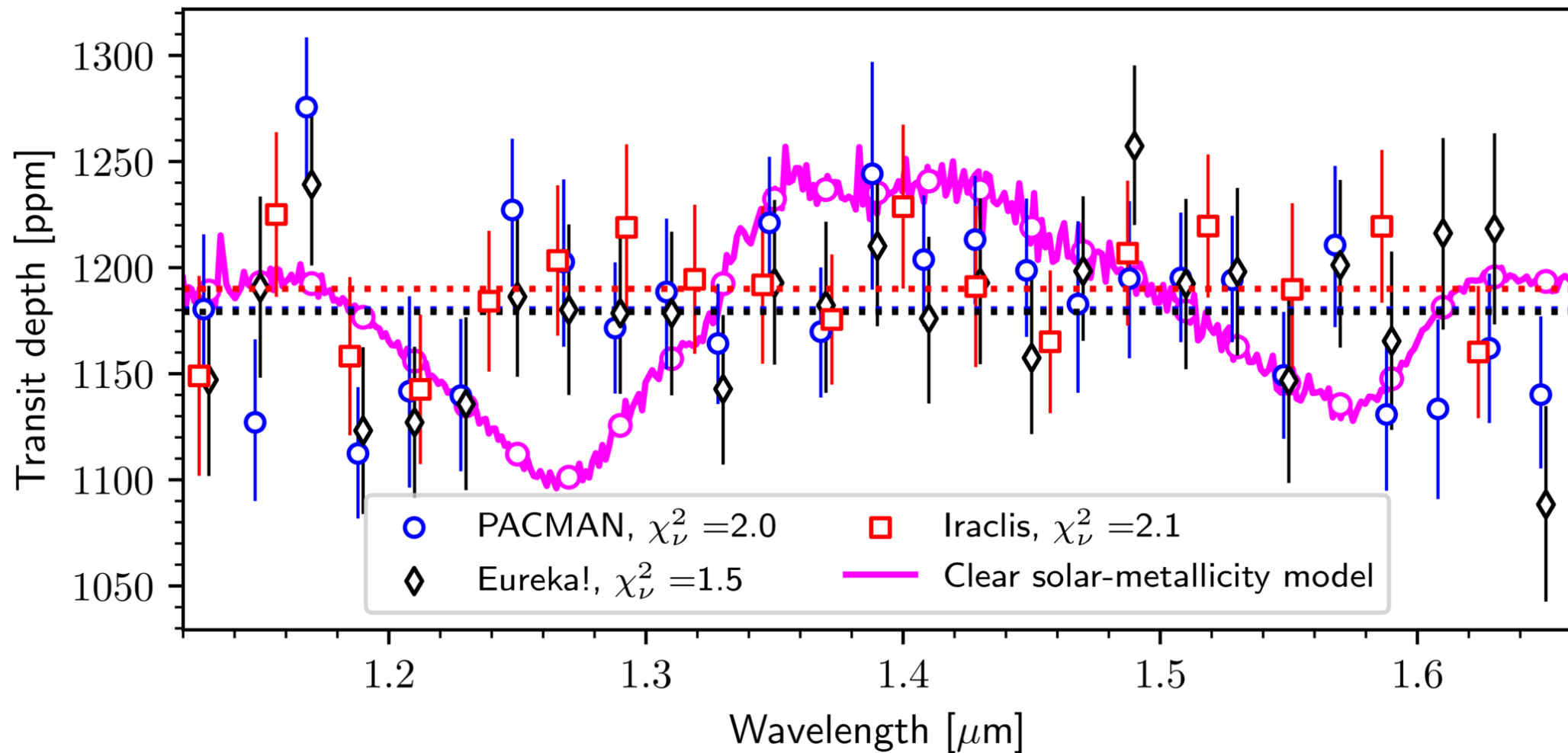
Figure 6. from Cyril Gapp et al 2026 Astron. J. 172 doi:10.3847/1538-3881/ae9866 https://dx.doi.org/10.3847/1538-3881/ae9866 © 2026. The Author(s). Published by the American Astronomical Society.
