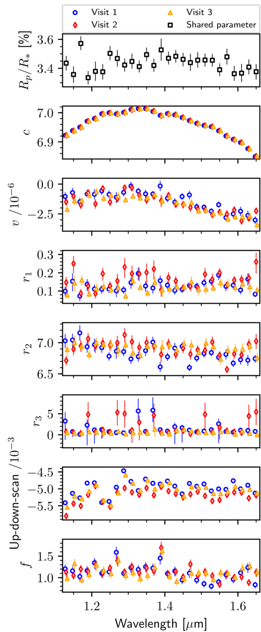
Figure 4. from Cyril Gapp et al 2026 Astron. J. 172 doi:10.3847/1538-3881/ae9866 https://dx.doi.org/10.3847/1538-3881/ae9866 © 2026. The Author(s). Published by the American Astronomical Society.
