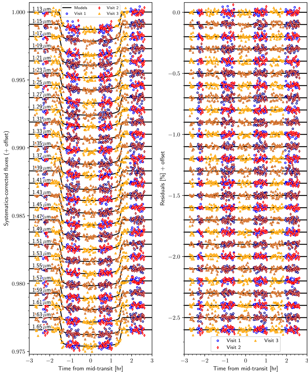
Figure 3. from Cyril Gapp et al 2026 Astron. J. 172 doi:10.3847/1538-3881/ae9866 https://dx.doi.org/10.3847/1538-3881/ae9866 © 2026. The Author(s). Published by the American Astronomical Society.
