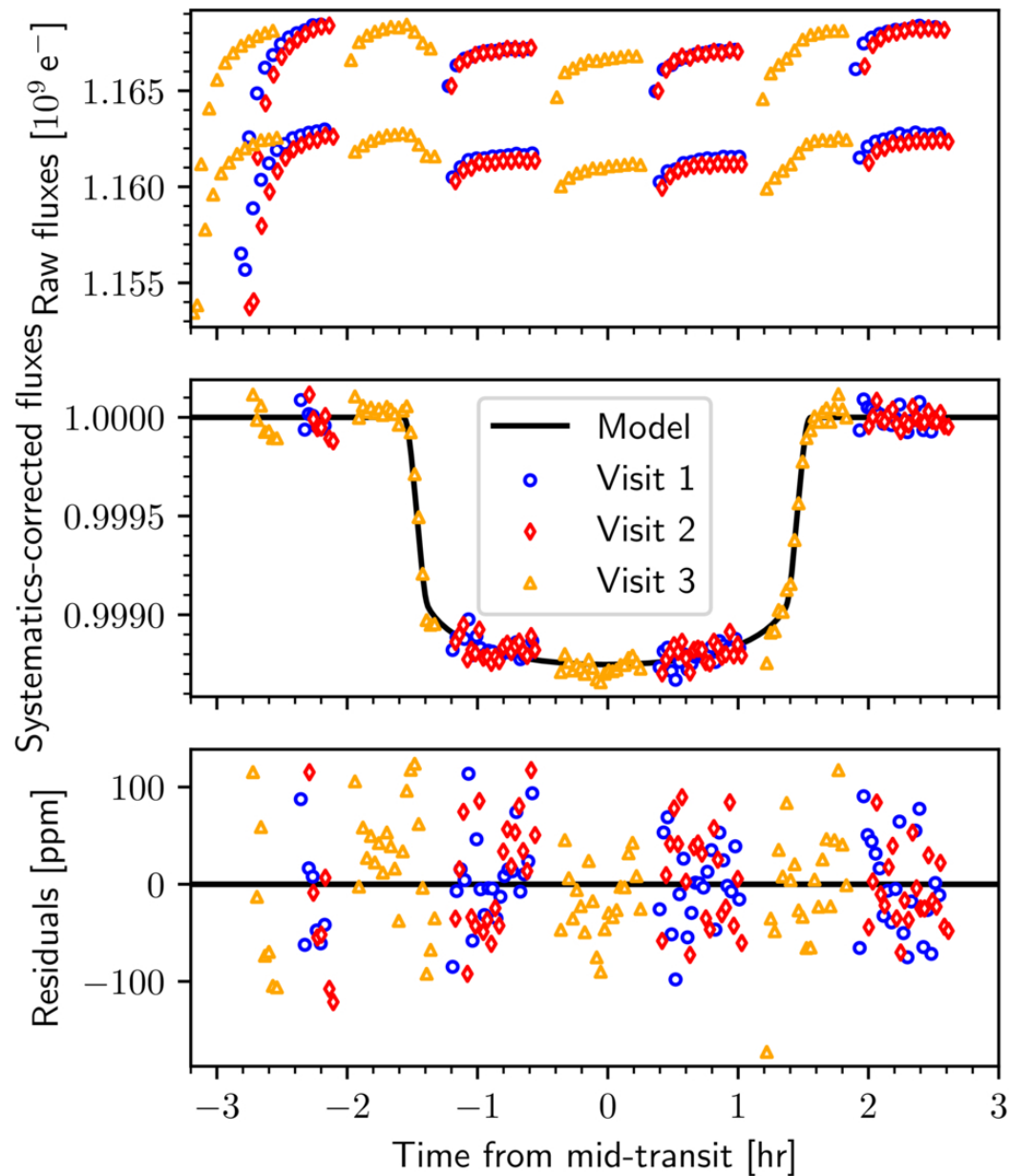
Figure 2. from Cyril Gapp et al 2026 Astron. J. 172 doi:10.3847/1538-3881/ae9866 https://dx.doi.org/10.3847/1538-3881/ae9866 © 2026. The Author(s). Published by the American Astronomical Society.
