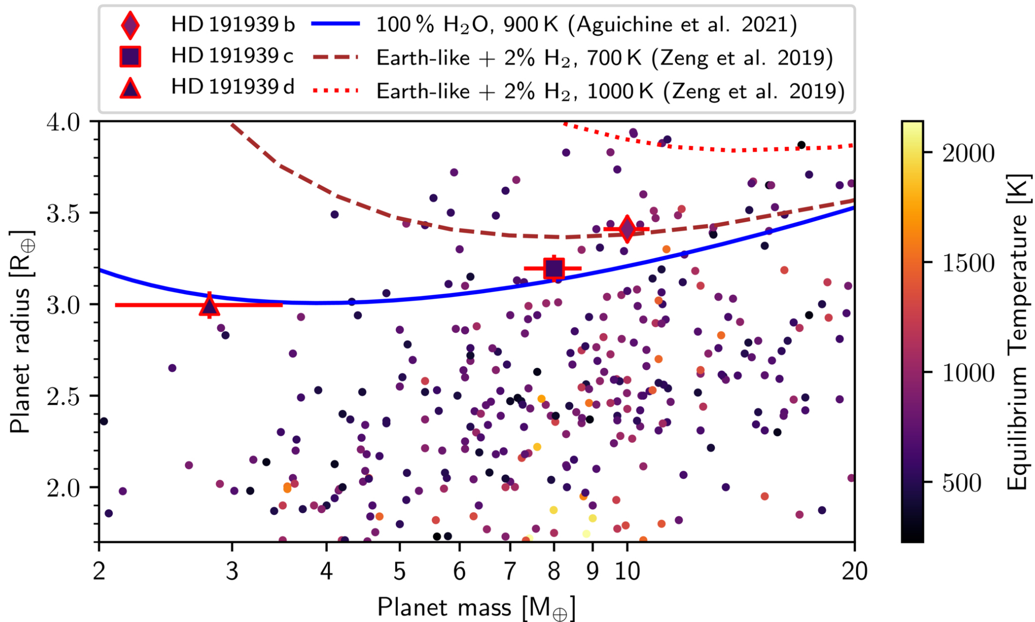
Figure 1. from Cyril Gapp et al 2026 Astron. J. 172 doi:10.3847/1538-3881/ae9866 https://dx.doi.org/10.3847/1538-3881/ae9866 © 2026. The Author(s). Published by the American Astronomical Society.
