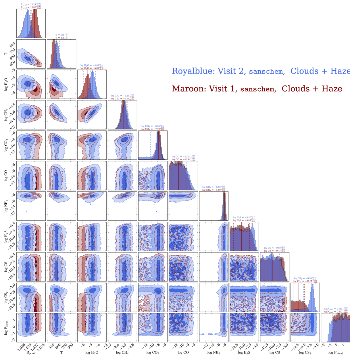
Figure 9. from Giannina Guzmán Caloca et al 2026 Astron. J. 172 doi:10.3847/1538-3881/ae9858 https://dx.doi.org/10.3847/1538-3881/ae9858 © 2026. The Author(s). Published by the American Astronomical Society.
