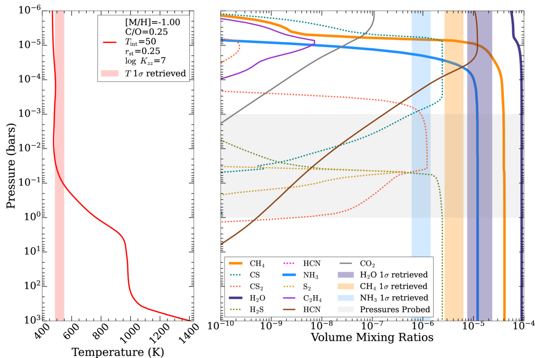
Figure 7. from Giannina Guzmán Caloca et al 2026 Astron. J. 172 doi:10.3847/1538-3881/ae9858 https://dx.doi.org/10.3847/1538-3881/ae9858 © 2026. The Author(s). Published by the American Astronomical Society.
