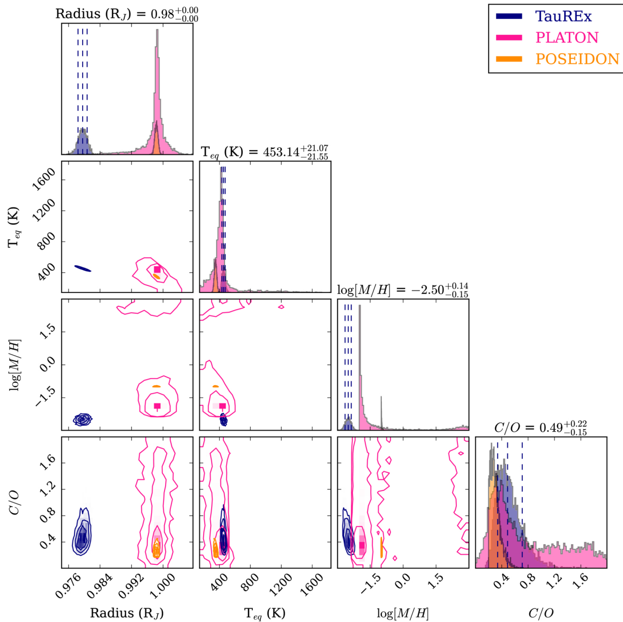
Figure 6. from Giannina Guzmán Caloca et al 2026 Astron. J. 172 doi:10.3847/1538-3881/ae9858 https://dx.doi.org/10.3847/1538-3881/ae9858 © 2026. The Author(s). Published by the American Astronomical Society.
