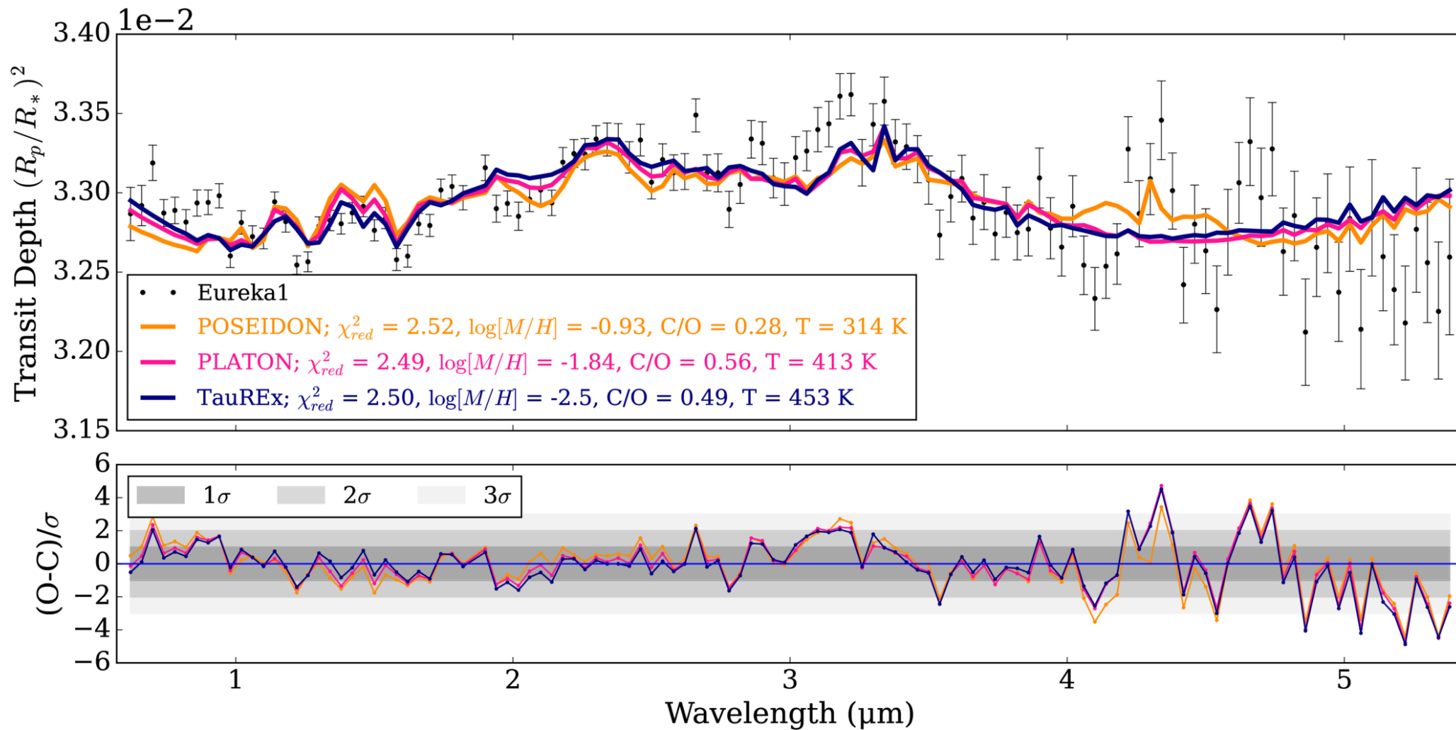
Figure 5. from Giannina Guzmán Caloca et al 2026 Astron. J. 172 doi:10.3847/1538-3881/ae9858 https://dx.doi.org/10.3847/1538-3881/ae9858 © 2026. The Author(s). Published by the American Astronomical Society.
