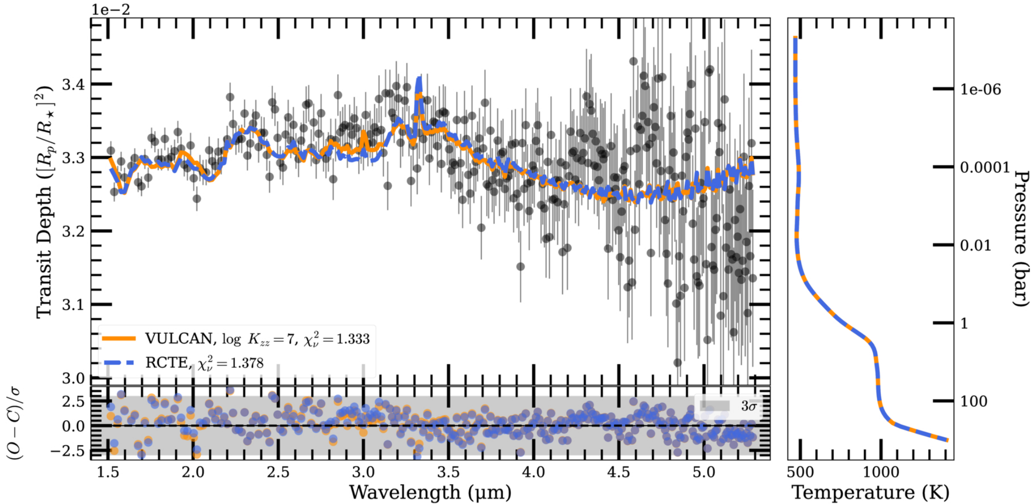
Figure 4. from Giannina Guzmán Caloca et al 2026 Astron. J. 172 doi:10.3847/1538-3881/ae9858 https://dx.doi.org/10.3847/1538-3881/ae9858 © 2026. The Author(s). Published by the American Astronomical Society.
