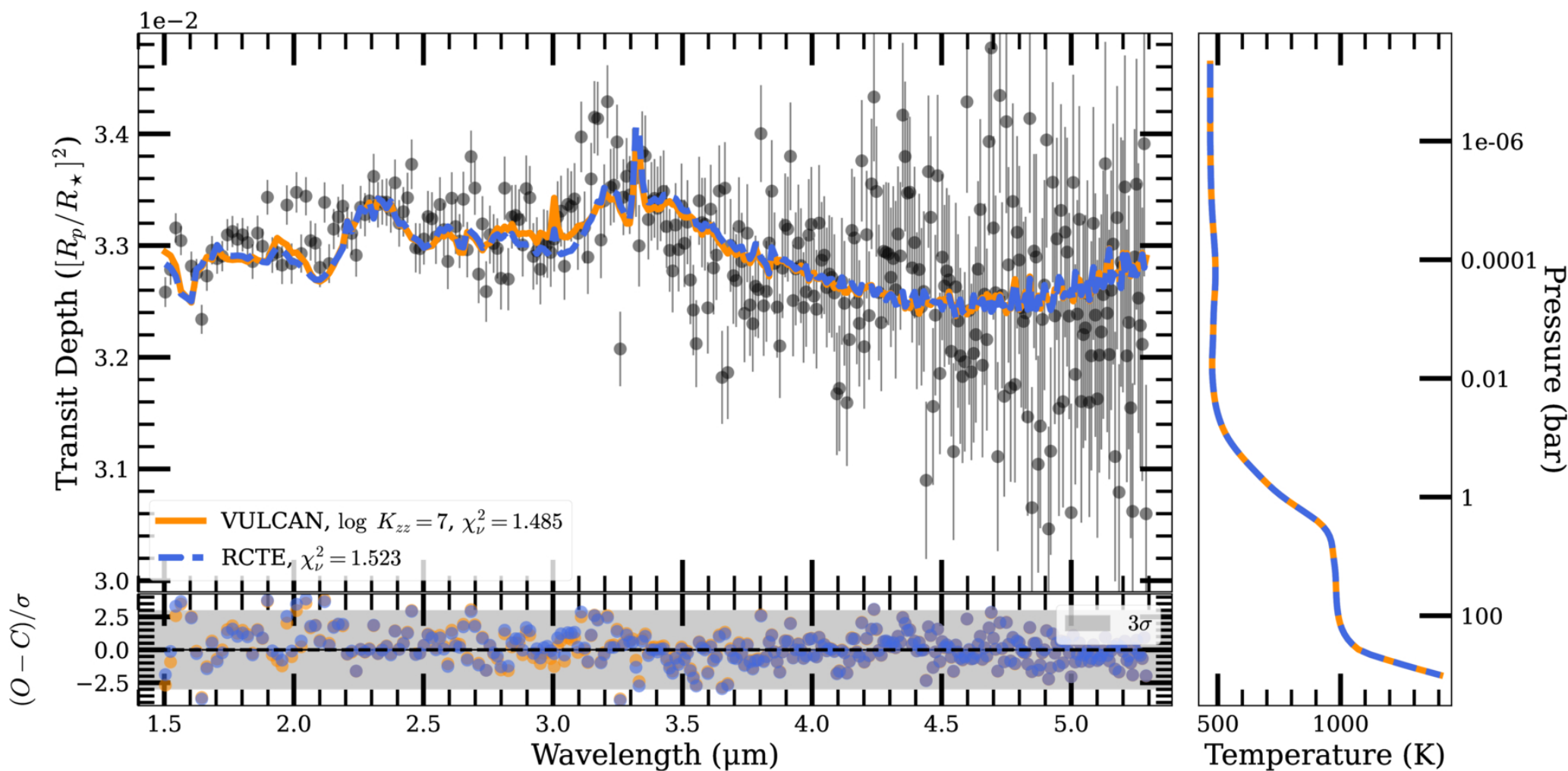
Figure 3. from Giannina Guzmán Caloca et al 2026 Astron. J. 172 doi:10.3847/1538-3881/ae9858 https://dx.doi.org/10.3847/1538-3881/ae9858 © 2026. The Author(s). Published by the American Astronomical Society.
