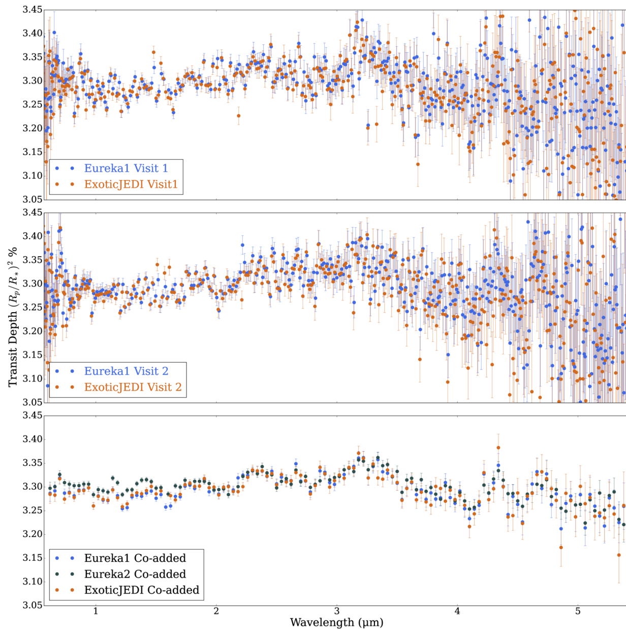
Figure 2. from Giannina Guzmán Caloca et al 2026 Astron. J. 172 doi:10.3847/1538-3881/ae9858 https://dx.doi.org/10.3847/1538-3881/ae9858 © 2026. The Author(s). Published by the American Astronomical Society.
