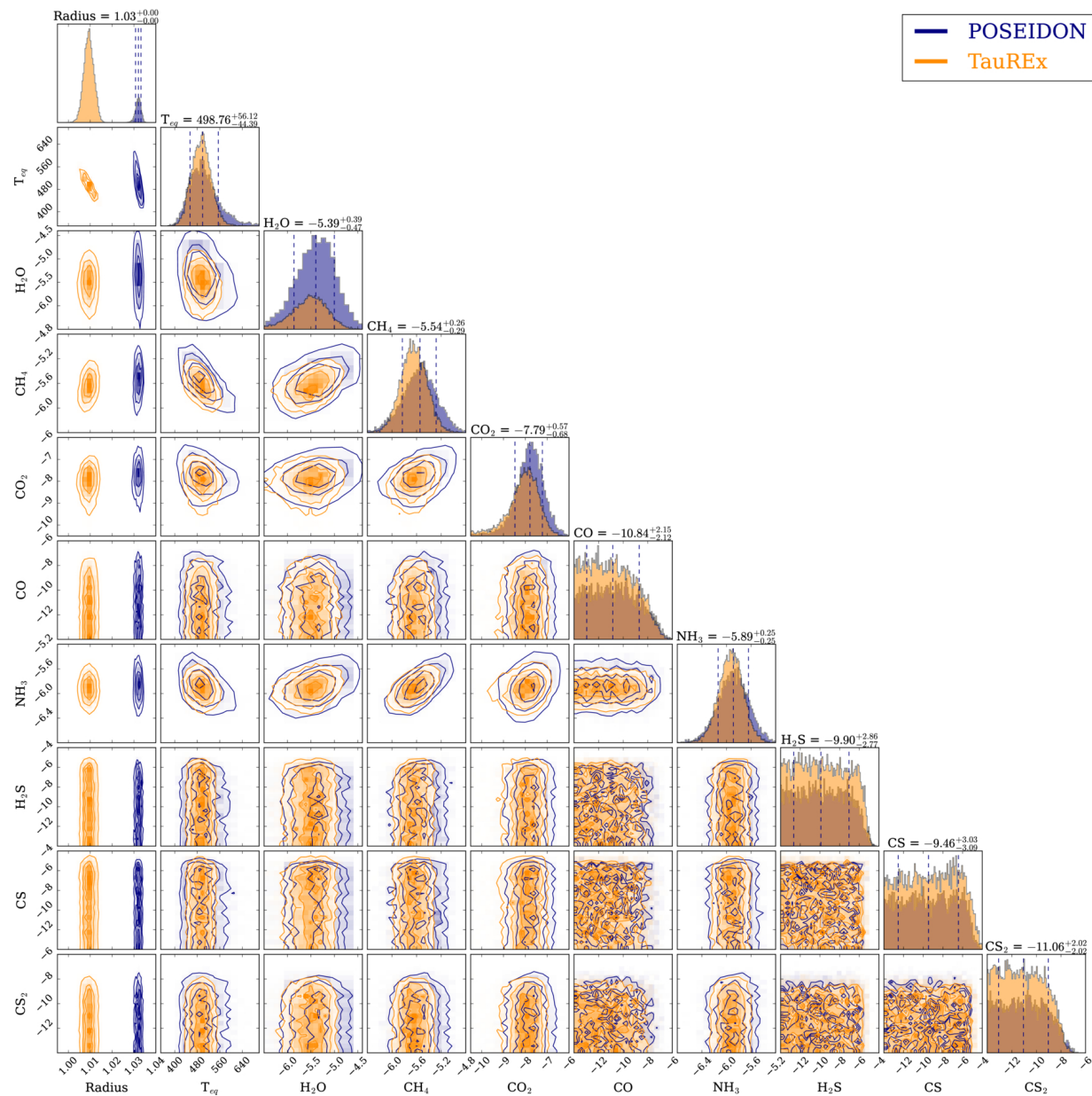
Figure 11. from Giannina Guzmán Caloca et al 2026 Astron. J. 172 doi:10.3847/1538-3881/ae9858 https://dx.doi.org/10.3847/1538-3881/ae9858 © 2026. The Author(s). Published by the American Astronomical Society.
