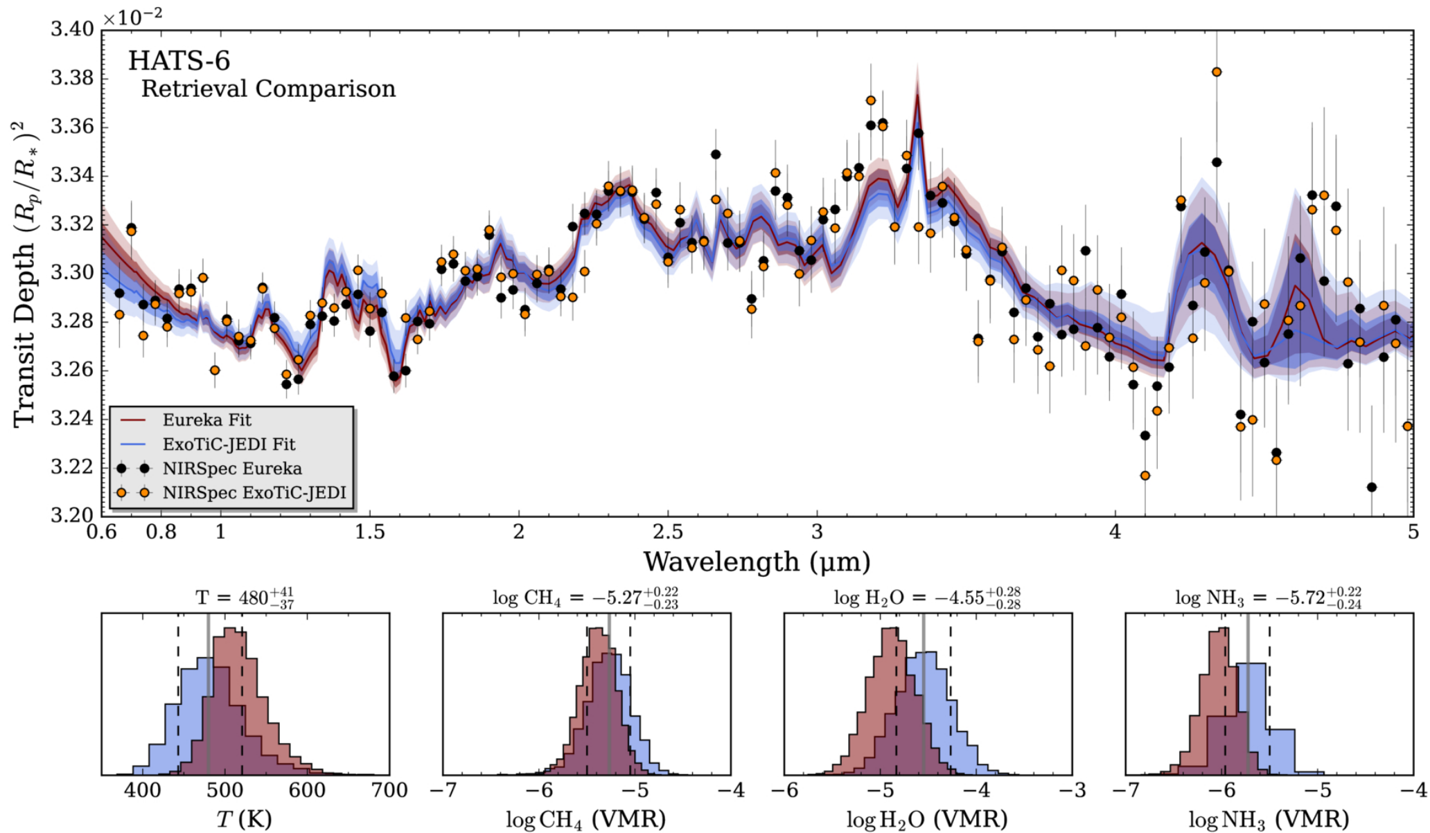
Figure 10. from Giannina Guzmán Caloca et al 2026 Astron. J. 172 doi:10.3847/1538-3881/ae9858 https://dx.doi.org/10.3847/1538-3881/ae9858 © 2026. The Author(s). Published by the American Astronomical Society.
