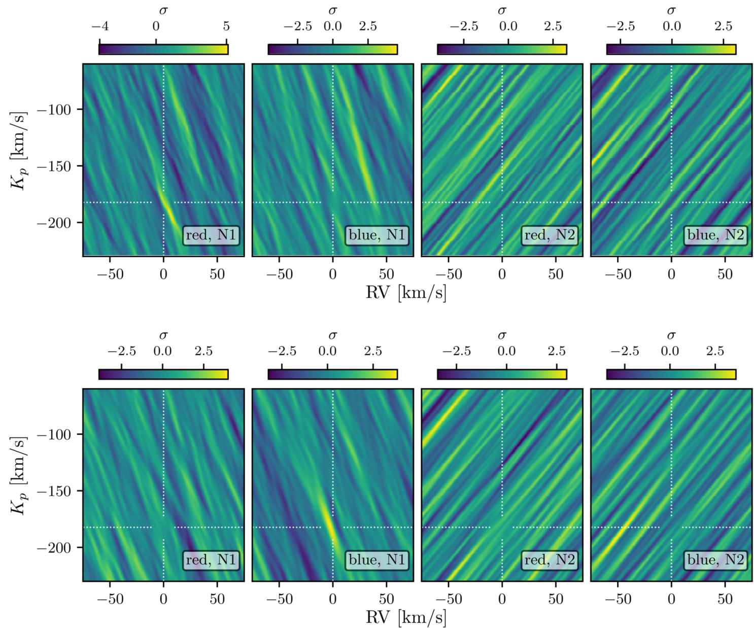
Figure 9. from Caitlin E. Bell et al 2026 Astron. J. 172 doi:10.3847/1538-3881/ae975e https://dx.doi.org/10.3847/1538-3881/ae975e © 2026. The Author(s). Published by the American Astronomical Society.
