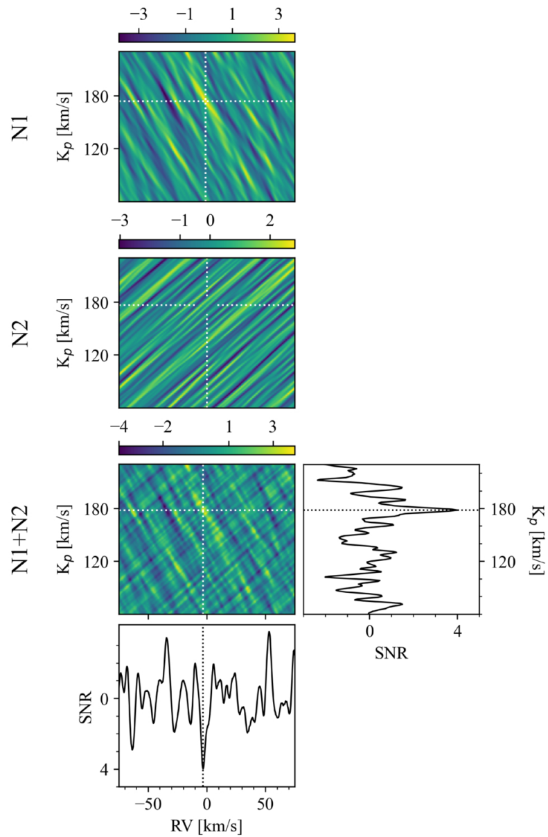
Figure 7. from Caitlin E. Bell et al 2026 Astron. J. 172 doi:10.3847/1538-3881/ae975e https://dx.doi.org/10.3847/1538-3881/ae975e © 2026. The Author(s). Published by the American Astronomical Society.
