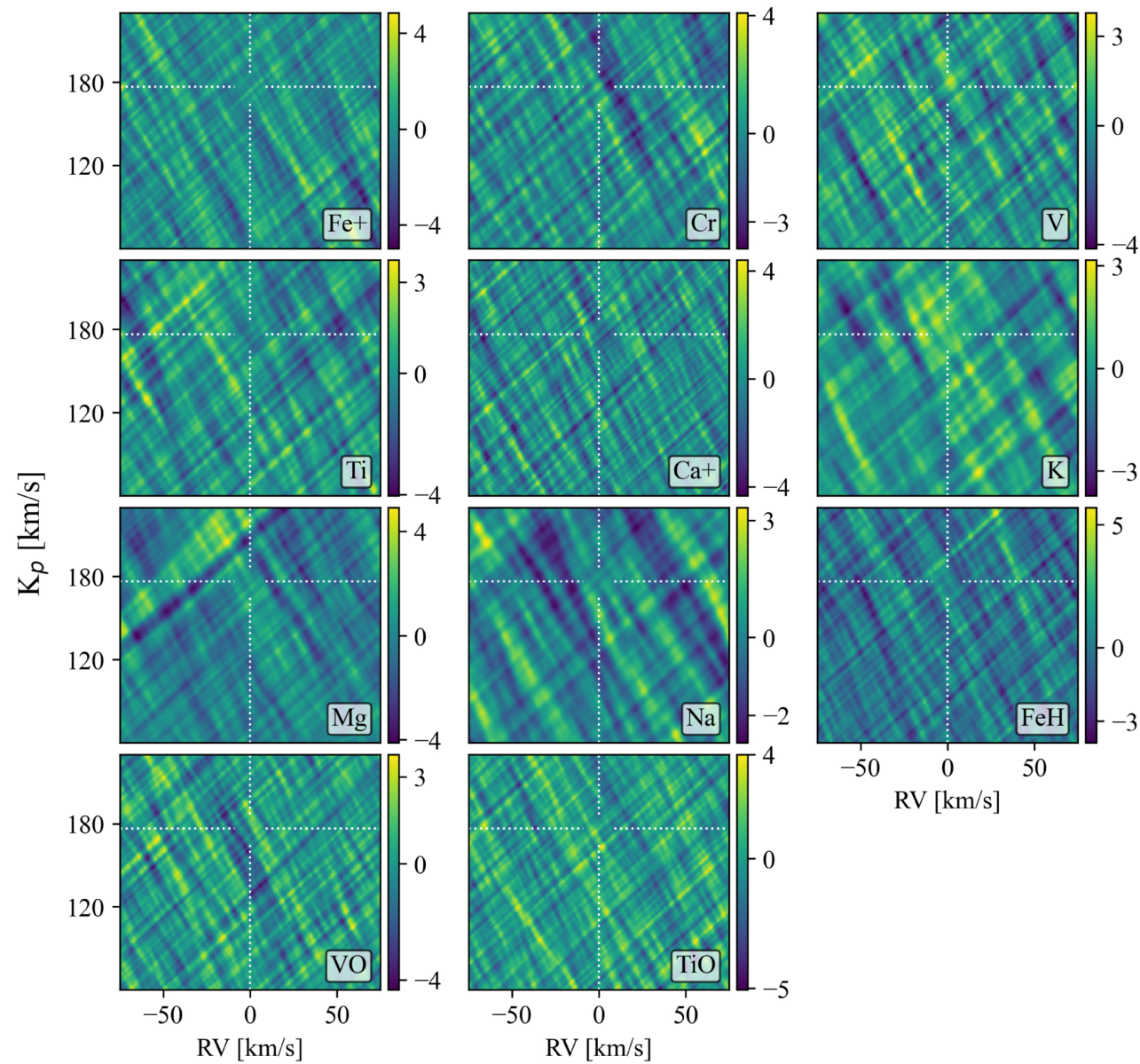
Figure 6. from Caitlin E. Bell et al 2026 Astron. J. 172 doi:10.3847/1538-3881/ae975e https://dx.doi.org/10.3847/1538-3881/ae975e © 2026. The Author(s). Published by the American Astronomical Society.
